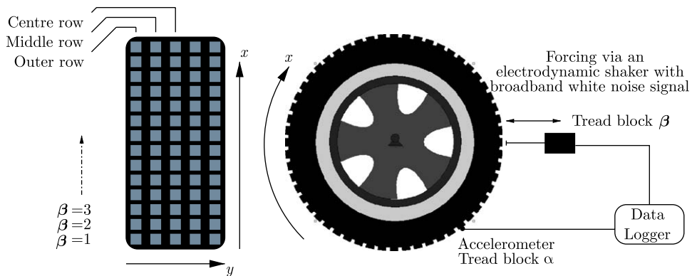
Fig. 9. Obtaining the transfer function between two tread blocks of a tyre. One block is forced at block \beta and the acceleration response obtained at block \alpha .
