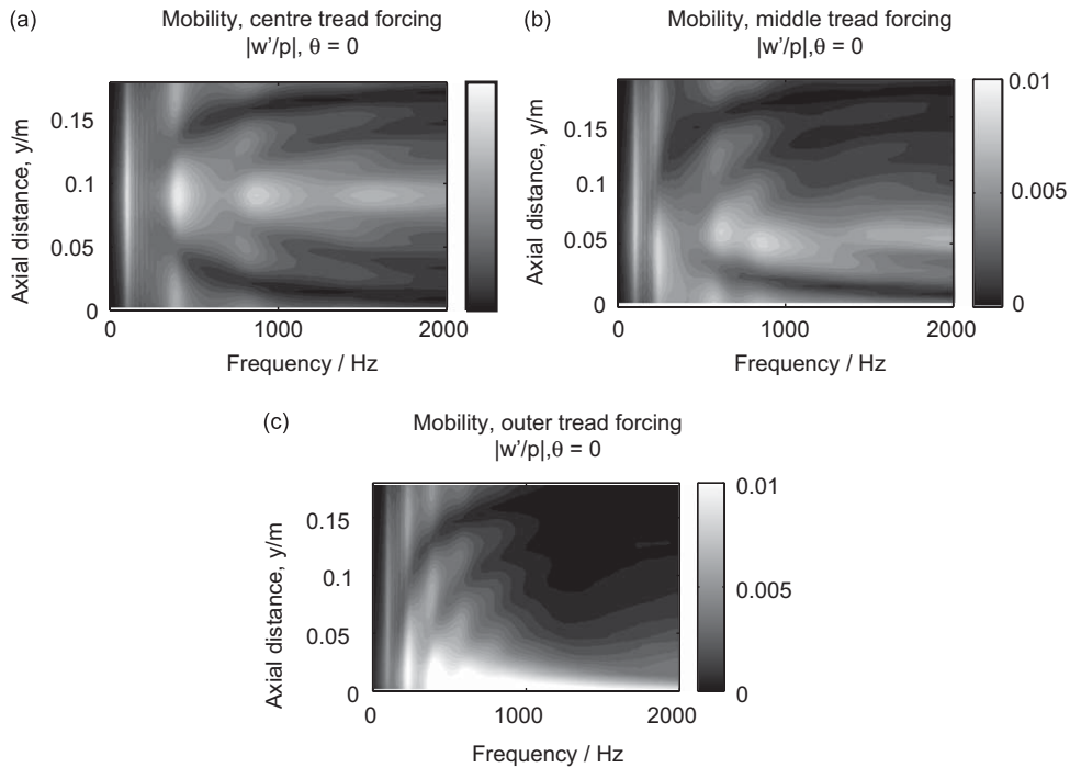
Fig. 12. Numerical mobility predictions, defined as the radial velocity response of the tyre surface, for an applied radial forcing. The mobility for the case where different rows of tread blocks are forced, as a function of frequency and axial position are shown for the circumferential position \theta = 0^\circ : (a) mobility where the centre row of tread blocks is excited; (b) the middle row of tread blocks is excited and (c) the outer row of tread blocks is excited.
