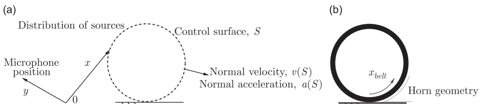
Fig. 18. The far-field sound is predicted by integrating individual sound sources over the surface of the tyre. The amplification due to the solid geometric shape of the tyre is then introduced via a transfer function: (a) distribution of sound sources on surface of tyre and (b) tyre geometry which leads to the horn amplification, where the circumferential position around the tyre is defined by x_{belt} . As x_{belt} increases, a diverging space is present, similar to a gramophone horn, which amplifies sound sources present.
