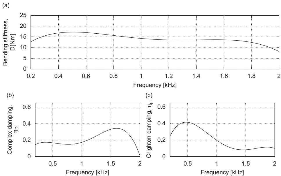
Fig. 7. Equivalent plate parameters for a viscoelastic tyre belt including a thick layer of tread rubber. (a) equivalent bending stiffness against frequency (Nm); (b) magnitude of the complex damping and (c) magnitude of Crighton damping.
