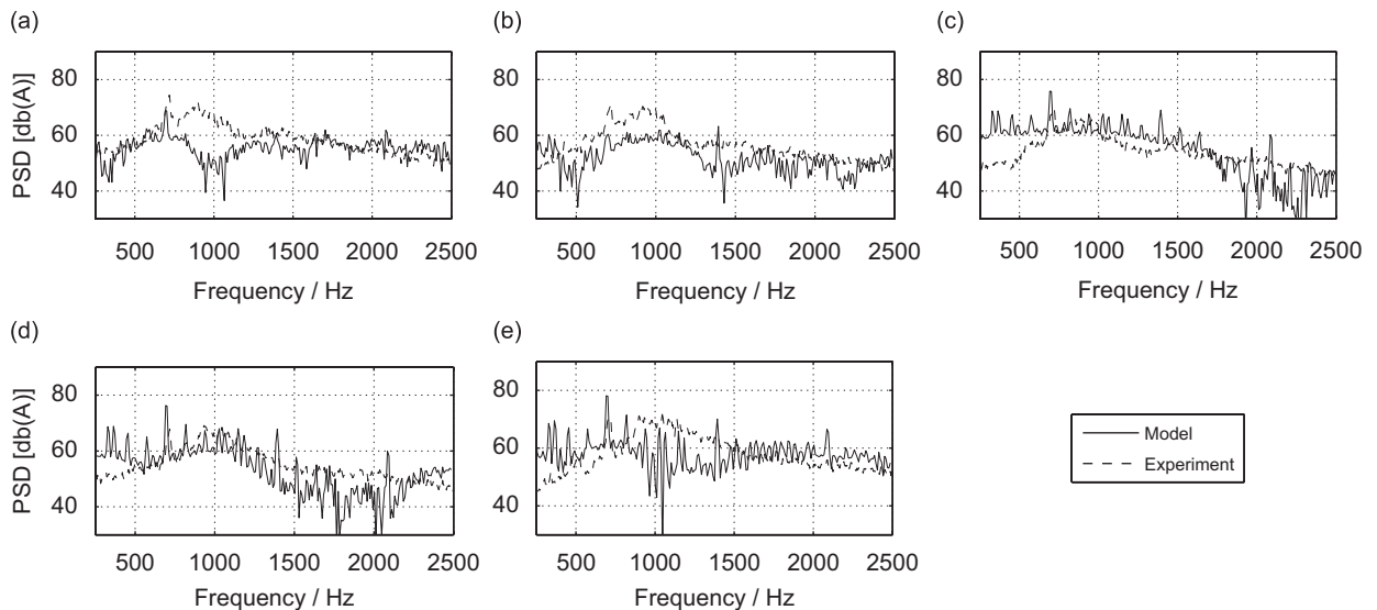
Fig. 23. Power spectral density of a patterned tyre rolling on a hot rolled asphalt road surface at 90 km/h. An A-weighting has been applied to both the predictions and experimental data: (a) microphone position 1; (b) microphone position 2; (c) microphone position 3; (d) microphone position 4 and (e) microphone position 5.
