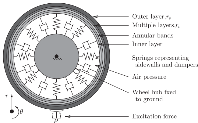
Fig. 1. Complete viscoelastic cylindrical model of the tyre belt.
