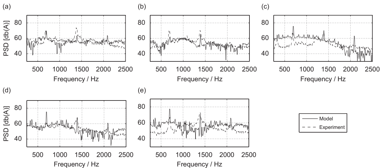
Fig. 21. Power spectral density of a patterned tyre rolling on a ISO-10844 specification road surface at 90 km/h. An A-weighting has been applied to both the predictions and experimental data: (a) microphone position 1; (b) microphone position 2; (c) microphone position 3; (d) microphone position 4 and (e) microphone position 5.
