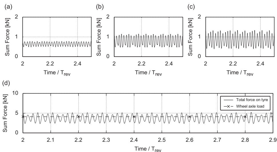
Fig. 15. Sum of the force on different rows of tread blocks for a tyre rolling on a smooth road surface with a forward speed of 80 km/h: (a) sum of the force on the outer row of tread blocks; (b) sum of the force on the middle row; (c) sum of the force on the centre row of tread blocks and (d) total predicted force on the tyre against static axle load applied to the tyre used for experimental measurements.
