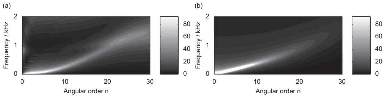
Fig. 8. Comparison of the velocity response of the viscoelastic tyre belt model with a thick layer of tread rubber, |\tilde{v}_r/\tilde{\sigma}_{rr}|[10^{-9}(\text{m}^3/\text{N})] with the equivalent plate |\tilde{w}/\tilde{p}|[10^{-9}(\text{m}^3/\text{N})] , for the m = 0 axial mode: (a) viscoelastic tyre belt and tread and (b) equivalent plate.
