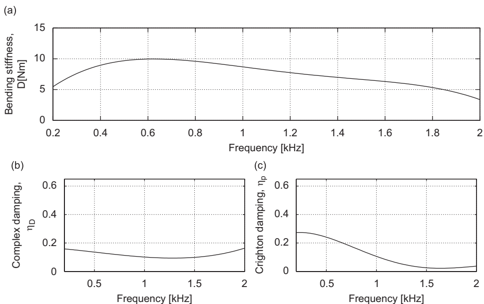
Fig. 5. Equivalent bending plate parameters for a viscoelastic tyre belt: (a) equivalent bending stiffness against frequency (N m), (b) magnitude of complex damping and (c) magnitude of the Crighton damping term.
