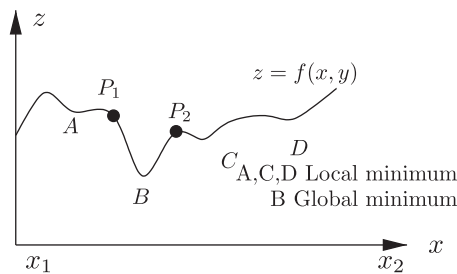
Fig. 3. Local and global minimum of function z = f(x, y) with initial starting point of error minimisation routine.
