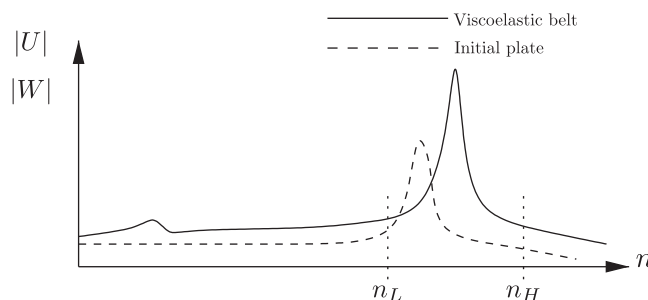
Fig. 4. Initial plate response before error minimisation. The response of the viscoelastic belt is illustrated, with a dominant flexural peak. The equivalent plate response should match the shape and amplitude of this peak, in addition to the low angular order amplitude.
