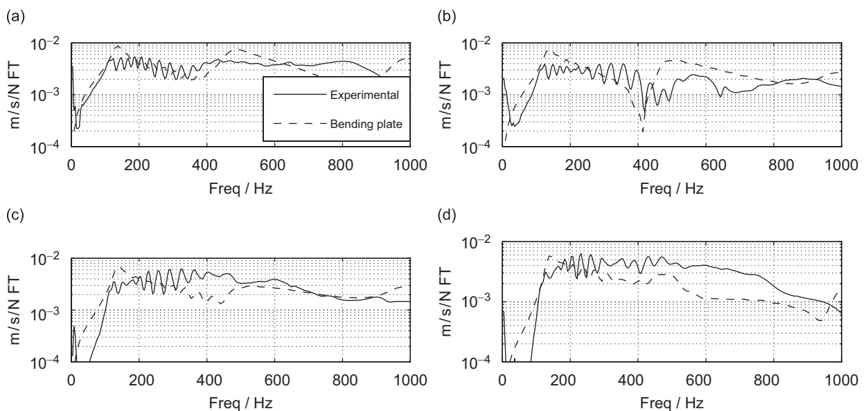
Fig. 11. Transfer functions showing radial velocity at tread block \alpha to radial harmonic forcing at tread block \beta for the centre row of tread blocks: (a) block \alpha = 2 ; (b) block \alpha = 3 ; (c) block \alpha = 4 and (d) block \alpha = 5 .
