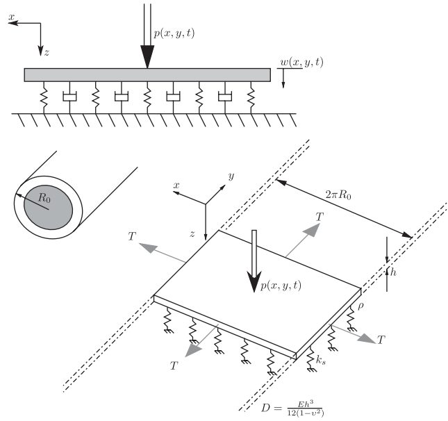
Fig. 2. Diagram of a thin bending plate with infinite width and in-plane tension, used for comparison to the viscoelastic multilayer tyre belt.
