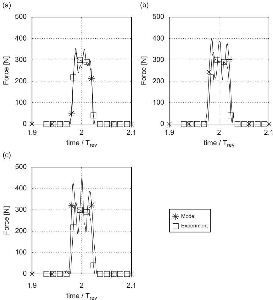
Fig. 16. Amplitude of the force on a tread block as it enters the contact patch compared with experimental data. The road surface is smooth with a patterned tyre rolling at 80 \text{ km/h} : (a) force profile for a tread block fixed to the outer row of tread blocks; (b) force profile for a block on the middle row and (c) force profile for a block on the centre row.
