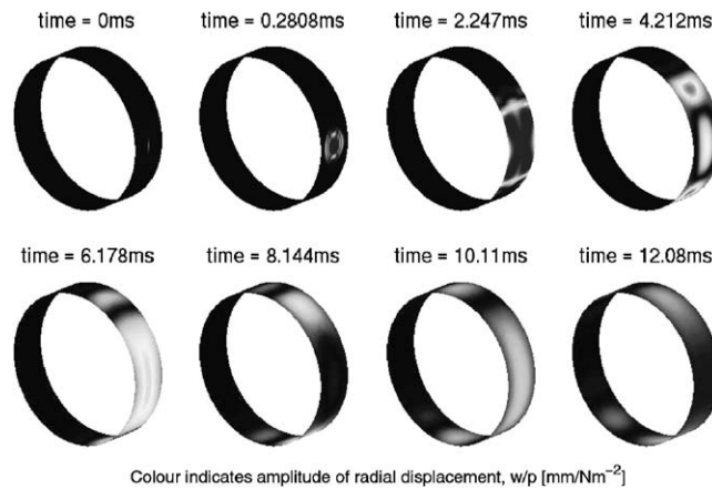
Fig. 13. Impulse response of the finite width tyre in the time domain, |w/p|[10^{-3}(\text{m}^3/\text{N})] , forcing a tread block in the centre row. Incremental time steps are shown with the colour gradient indicating the amplitude of the response (the predictions for the bending plate have been superimposed onto a cylindrical shape).
