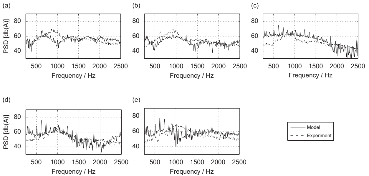
Fig. 22. Power spectral density of a patterned tyre rolling on a hot rolled asphalt road surface at 80 km/h. An A-weighting has been applied to both the predictions and experimental data: (a) microphone position 1; (b) microphone position 2; (c) microphone position 3; (d) microphone position 4 and (e) microphone position 5.
