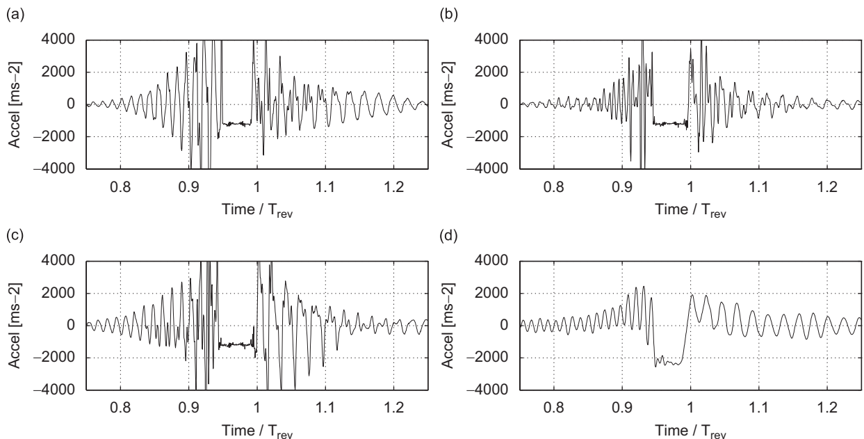
Fig. 17. Comparison of the acceleration of a tread block on each tread row, entering and leaving the contact patch, with experimental data. The road surface is smooth with a patterned tyre rolling at 80 km/h: (a) acceleration of a block from the outer row of tread blocks; (b) acceleration of a block from the middle row of tread blocks; (c) acceleration of a block from the centre row of tread blocks and (d) experimentally measured tread block acceleration.
