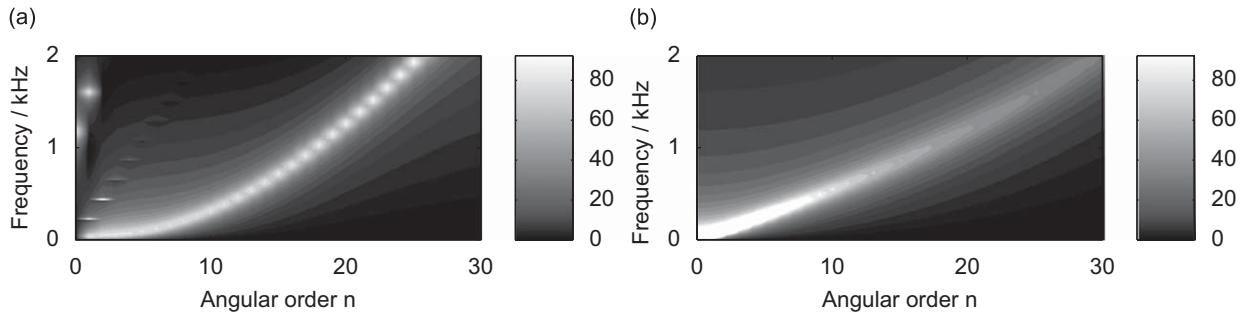
Fig. 6. Comparison of the velocity response of the viscoelastic tyre belt model without a thick layer of tread rubber, |\tilde{v}_r/\tilde{\sigma}_{rr}|[10^{-9}(\text{m}^3/\text{N})] with the equivalent plate |\tilde{w}/\tilde{p}|[10^{-9}(\text{m}^3/\text{N})] for the m = 0 axial mode of vibration: (a) Viscoelastic tyre belt and (b) equivalent plate.
