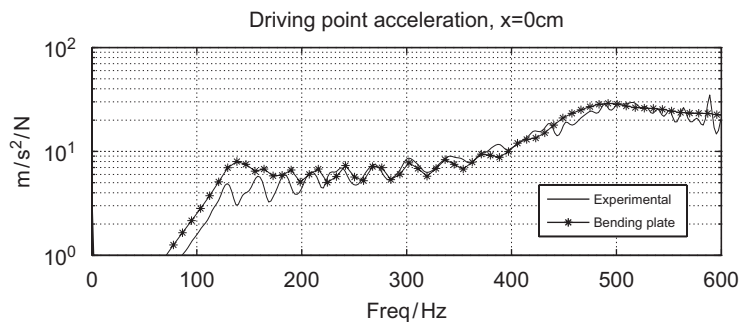
Fig. 10. Point accelerance showing radial acceleration at a tread block to radial harmonic forcing at the same tread block for the centre row of tread blocks.
