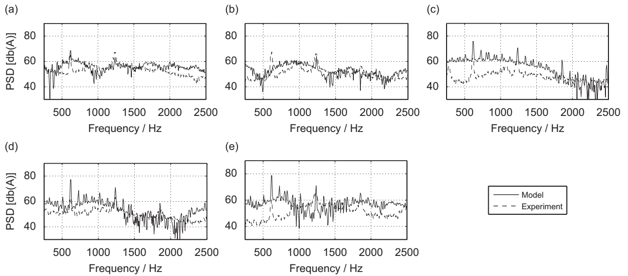
Fig. 20. Power spectral density of a patterned tyre rolling on a ISO-10844 specification road surface at 80 km/h. An A-weighting has been applied to both the predictions and experimental data: (a) microphone position 1; (b) microphone position 2; (c) microphone position 3; (d) microphone position 4 and (e) microphone position 5.
