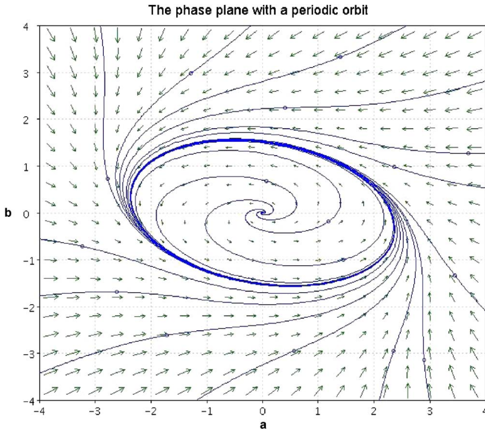
Fig. 6. The phase plane of the system (4) has been drawn for \alpha_0 = 1, \beta_0 = 1, \omega_0 = 1, h_0 = 2 and d = 1 . In this case, 2|d| > h_0\omega_0/2 so no nontrivial equilibrium points exist. The quadric, which is an ellipse for these parameter values, is clearly visible. All drawn solutions converge to the periodic elliptical orbit.
