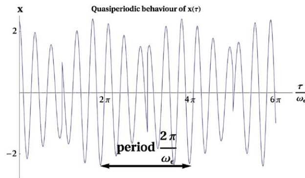
Fig. 3. The quasiperiodic behaviour of x(\tau) . The function is plotted for \alpha_0 = 1 , \beta_0 = 1 , h_0 = 2 , \omega_0 = 2 and d = 1 , while \varepsilon = 0.1 . Since 2|d| > h_0 \omega_0 / 2 , a and b exhibit periodic behaviour. This period of order 1/\varepsilon is indicated in the figure. The initial frequency of order 1 is also visible.
