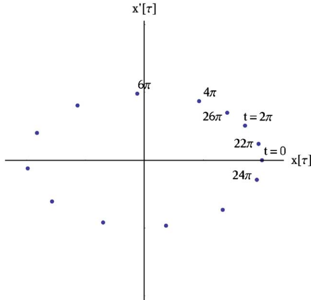
Fig. 4. The Poincaré section (also known as the “time = 2π”-map or stroboscopic map) based on the original system (1), of the quasiperiodic solution of x(\tau) in phase space (x(\tau), x'(\tau)) . The first 13 iterations are shown. In this plot, \omega_0 = 1 .
