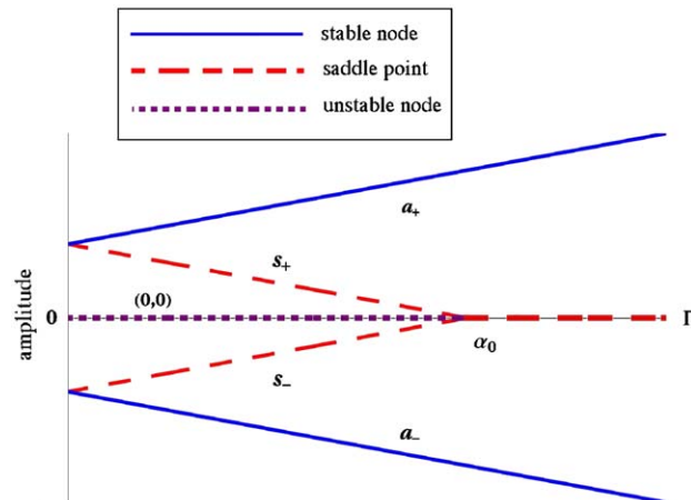
Fig. 1. Bifurcation analysis of the equilibrium points of the system of equation (4). The points of the symmetric pair are indicated by s_\pm and those of the antisymmetric pair by a_\pm . The relevant bifurcation parameter is \Gamma = \sqrt{(h_0^2 \omega_0^2 / 4) - 4d^2} . We see that if \Gamma < \alpha_0 , four nontrivial equilibrium points exist while the origin is an unstable node. For \Gamma > \alpha_0 , only two nontrivial equilibrium points exist; the origin has turned into a saddle point. We can therefore identify a subcritical pitchfork bifurcation at \Gamma = \alpha_0 and two simultaneous saddle-node bifurcations at \Gamma = 0 .
