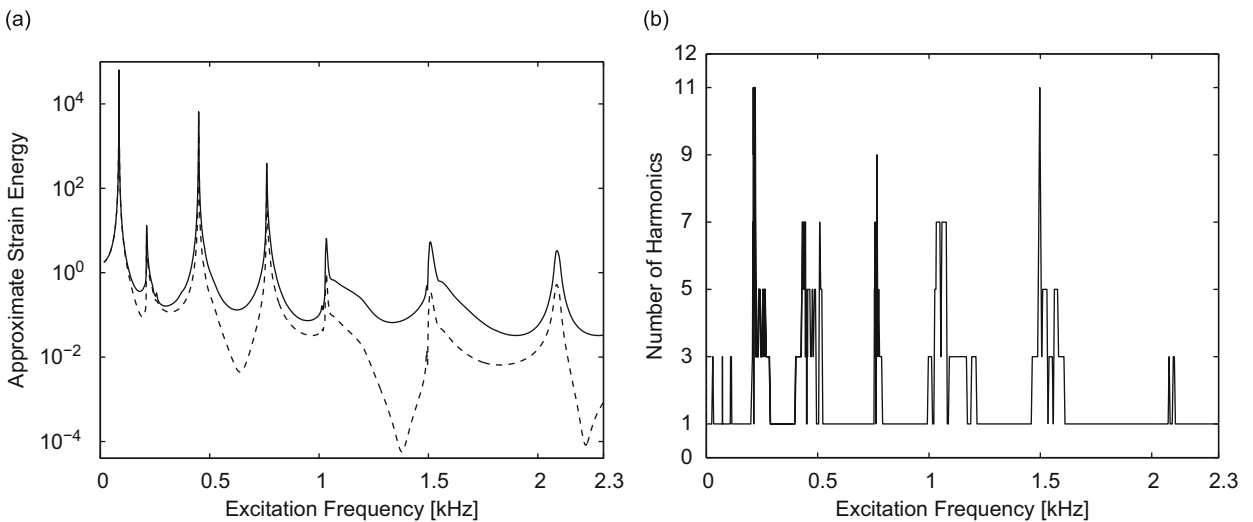
Fig. 14. (a) Approximate strain energy: — general expression; - - condensation case expression. (b) Number of harmonics obtained with the condensation case expression.
