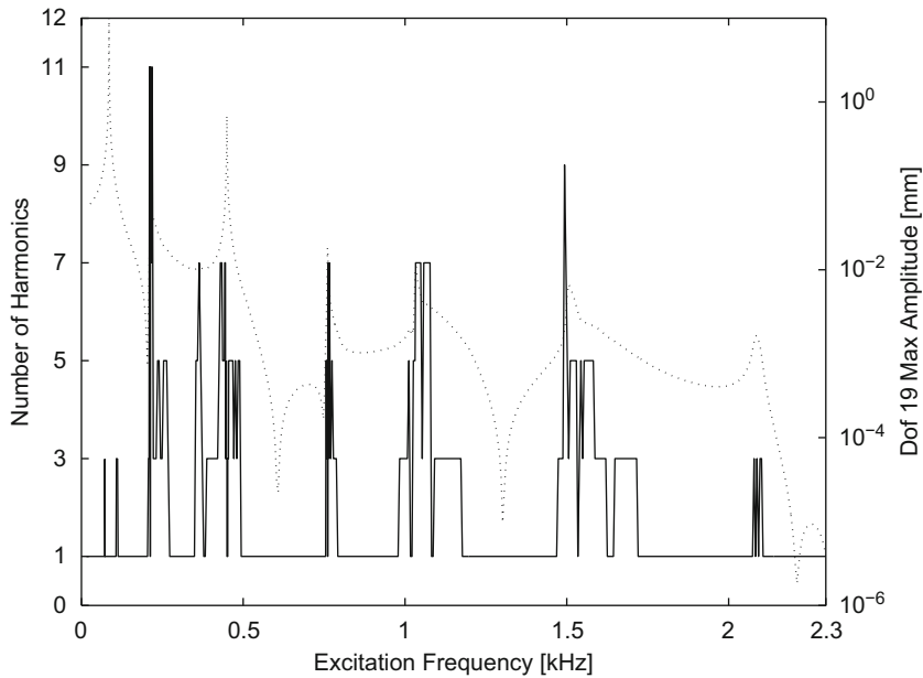
Fig. 5. Evolution of the number of harmonics: — number of harmonics; ... maximal amplitude of vibration for dof 19.
