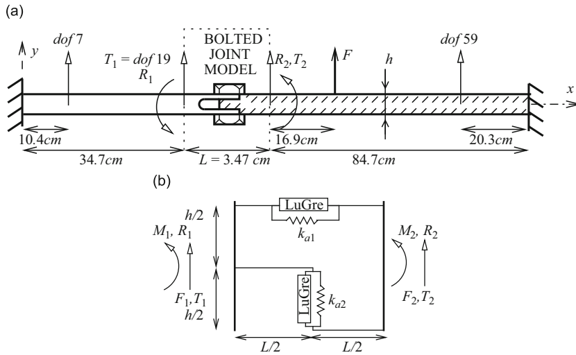
Fig. 3. Application case (a) two beam system and (b) bolted joint model.
