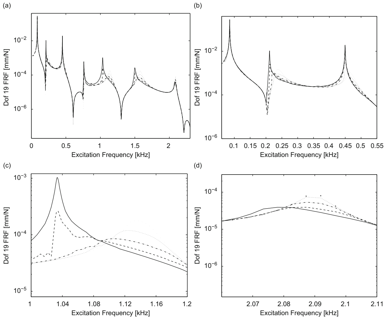
Fig. 11. Influence of excitation force amplitude on frequency response functions for dof 19: (a) over all the frequency band, (b) zoom on three first resonances, (c) zoom on 1.1 kHz resonance, (d) zoom on 2 kHz resonance: ... (replaced by ++ on (d)) 6 N; - - - 12 N; -.- 24 N; - - 42 N; — 66 N.
