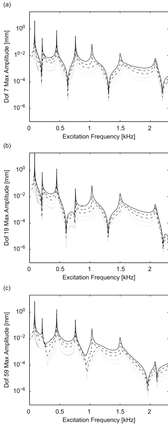
Fig. 9. Influence of excitation force amplitude on maximal amplitude of vibration for dofs 7(a), 19(b), 59(c): ... 6 N; - - - 12 N; -.- 24 N; - - - 42 N; — 66 N.
