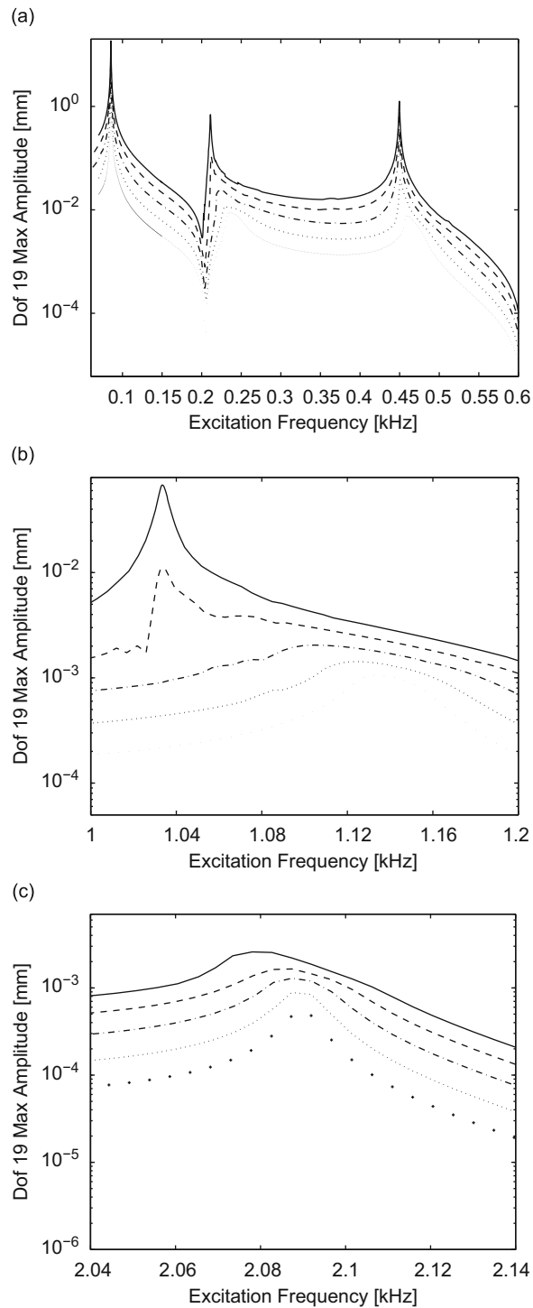
Fig. 10. Influence of excitation force amplitude on maximal amplitude of vibration for dof 19: (a) zoom on 3 first resonances, (b) zoom on 1.1 kHz resonance and (c) zoom on 2 kHz resonance: ... (replaced by ++ on (c)) 6 N; - - - 12 N; - · - 24 N; - - - 42 N; — 66 N.
