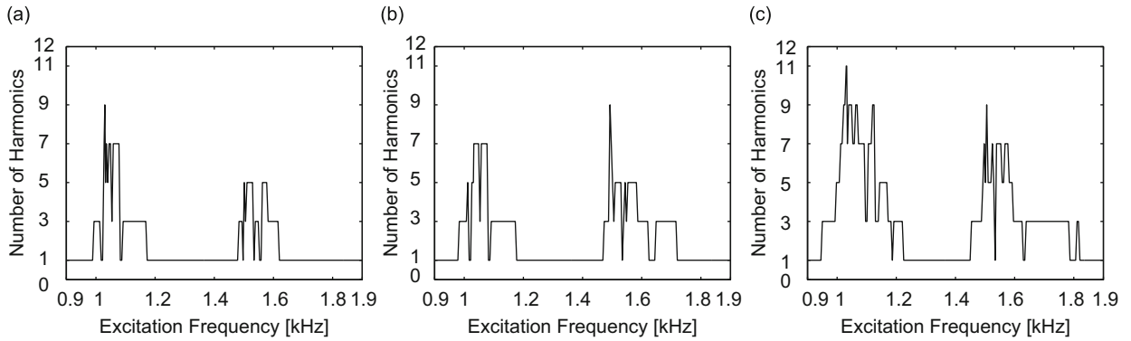
Fig. 13. Influence of threshold value on the number of harmonics, zoom on the 1.1 kHz and the 1.5 kHz resonances: (a) 5 percent, (b) 3 percent and (c) 1 percent.
