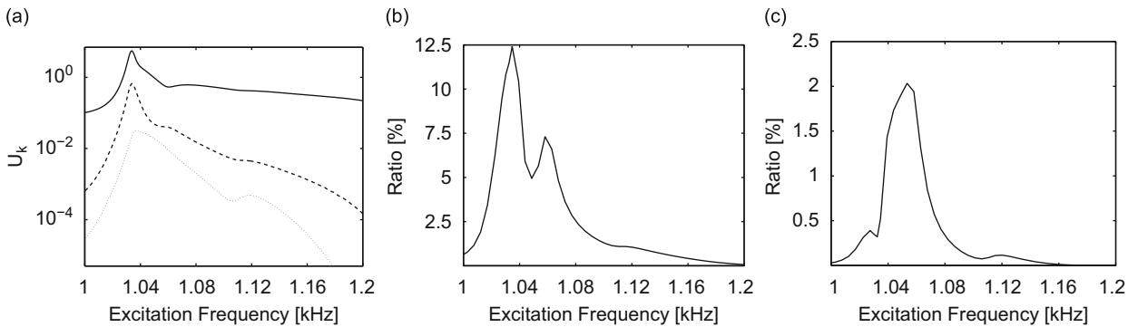
Fig. 7. Contribution of 1st, 3rd and 5th harmonics on approximate strain energy and associated ratios: (a) contribution of the: — 1st harmonic; – – 3rd harmonic; ... 5th harmonic; (b) ratio 3rd/1st; (c) ratio 5th/1st.
