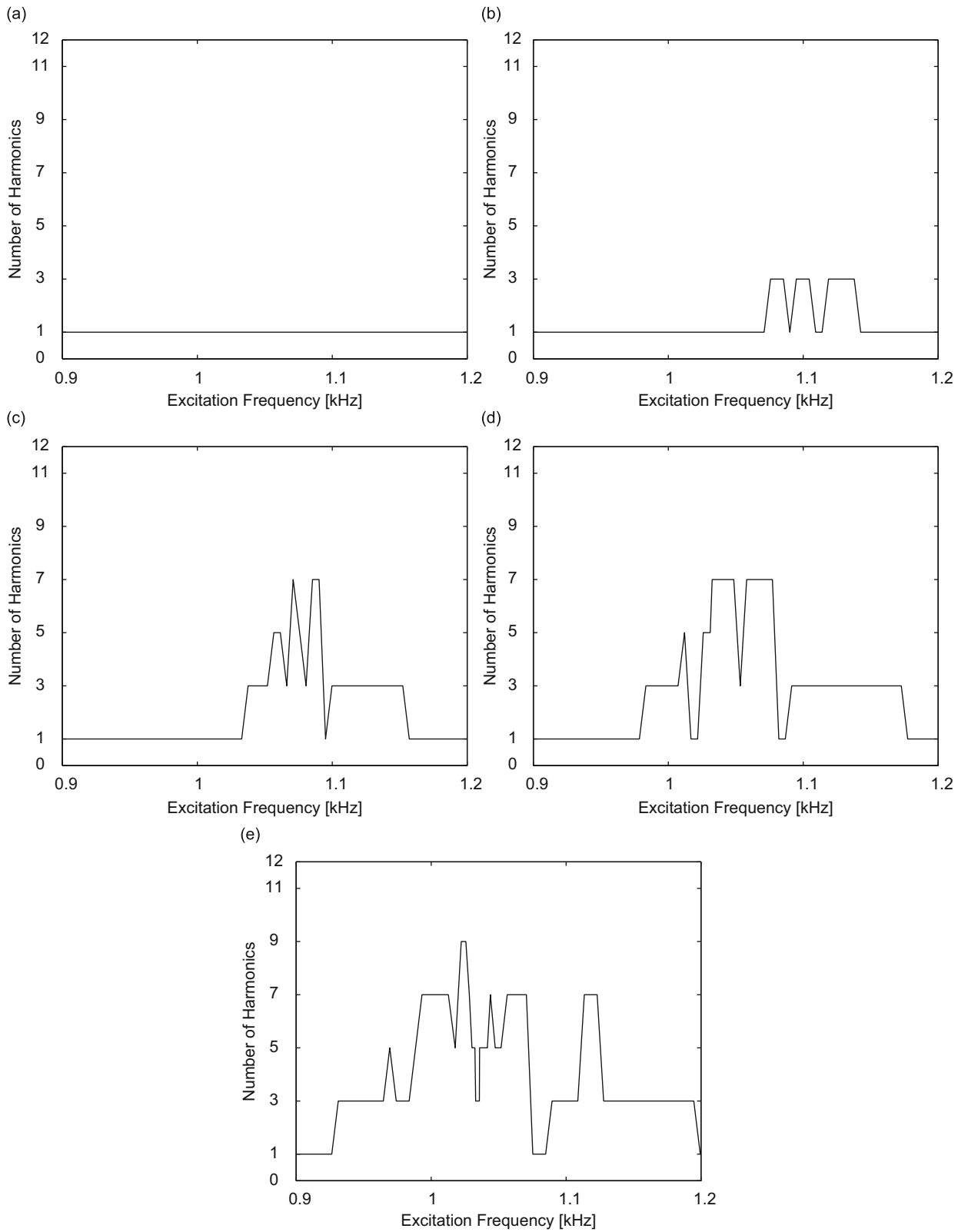
Fig. 12. Influence of excitation force amplitude on the number of harmonics, zoom on the 1.1 kHz resonance: (a) 6 N, (b) 12 N, (c) 24 N, (d) 42 N and (e) 66 N.
