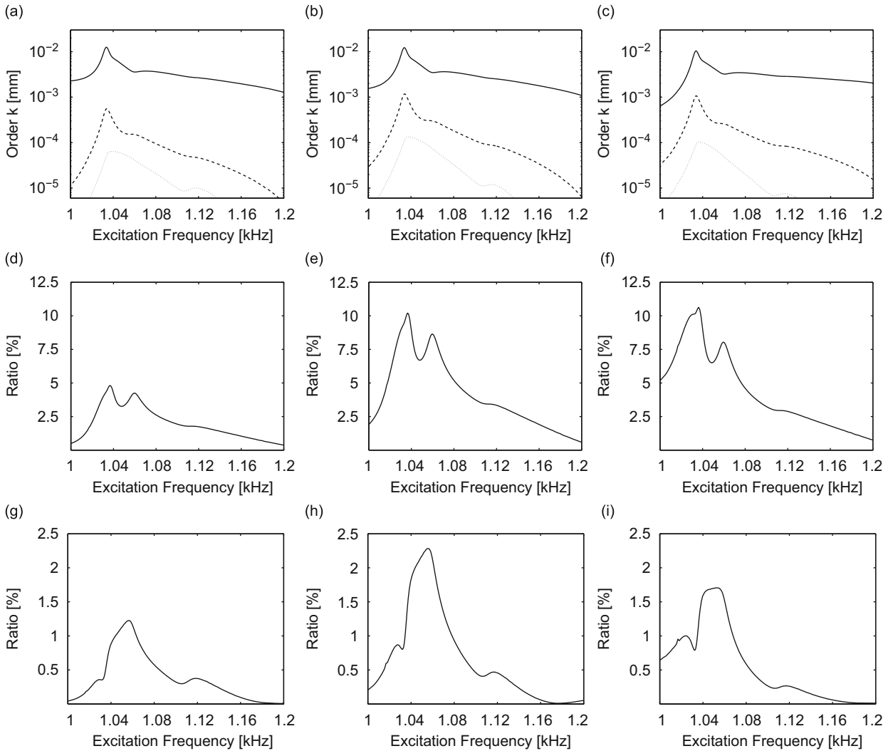
Fig. 6. Contribution of 1st, 3rd and 5th harmonics on maximal amplitude of vibration and associated ratios for dofs 7(a, d, g), 19(b, e, h), 59(c,f,i): (a–c) Fourier coefficient modulus of the: — 1st harmonic; – – 3rd harmonic; ... 5th harmonic; (d–f) ratio 3rd/1st; (g–i) ratio 5th/1st.
