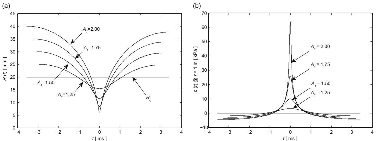
Fig. 1. (a) Computed time plots of bubble radius R(t) for different amplitudes of oscillations A_1 . (b) Computed time plots of radiated acoustic pressures p(t) for different amplitudes of oscillation A_1 .
