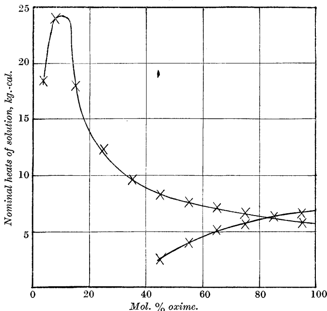
Nominal heats of solution in benzene : rising curve, \alpha -oxime ; falling curve, \beta -oxime.
