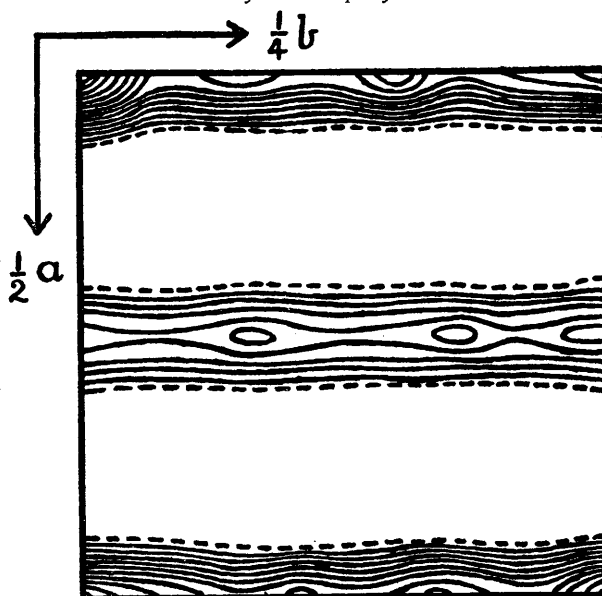
Patterson-Fourier projection on (001) showing high ridges separated by \frac{1}{3}a (7 Å.), and lower ridge half way between.
