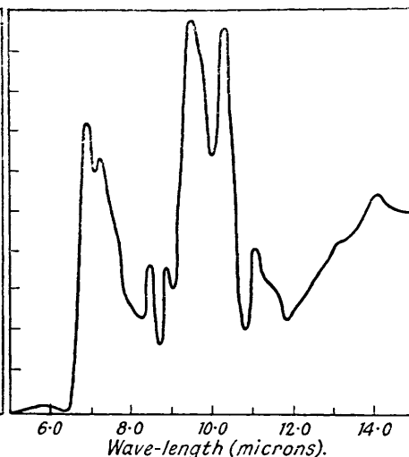
FIG. 2. trans-Hex-3-enol.
