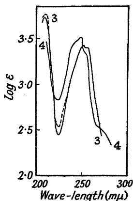
FIGS. 7—8. (7) 2-Methylthio-; (8) 2-methoxypyrimidine.
