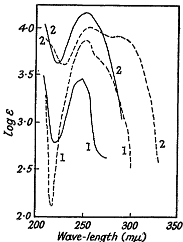
FIGS. 5—6. (5) 5-Chloro-; (6) 5-bromo-pyrimidine.
