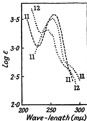
FIGS. 11—12. (11) Pyrimidine-4 ; (12) pyrimidine-5-carboxylic acid .
