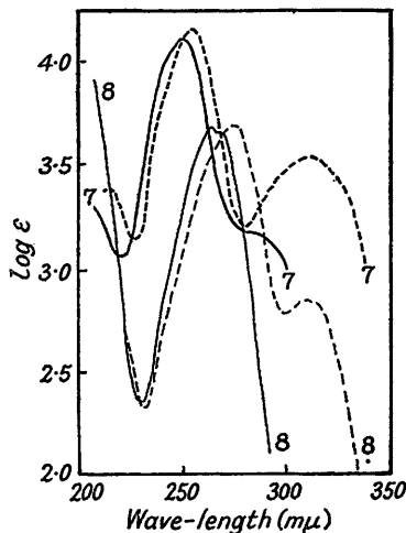
FIGS. 7—8. (7) 2-Methylthio-; (8) 2-methoxypyrimidine.
