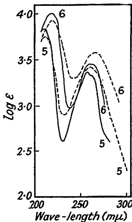
FIGS. 5—6. (5) 5-Chloro-; (6) 5-bromo-pyrimidine.
