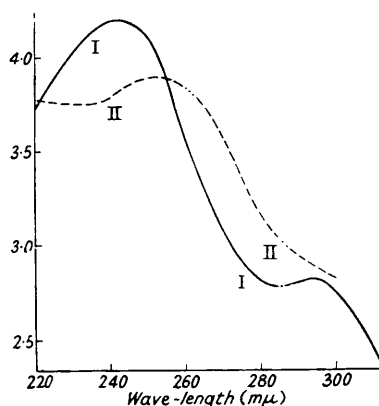
I, p -Benzoquinone. II, 5:6-Dibromocyclohex-2-ene-1:4-dione.
