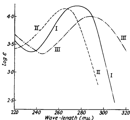
I, Aurantiogliocladin. II, 3:4-Dimethoxy-2:5-toluquinone. III, Gliorosein.
