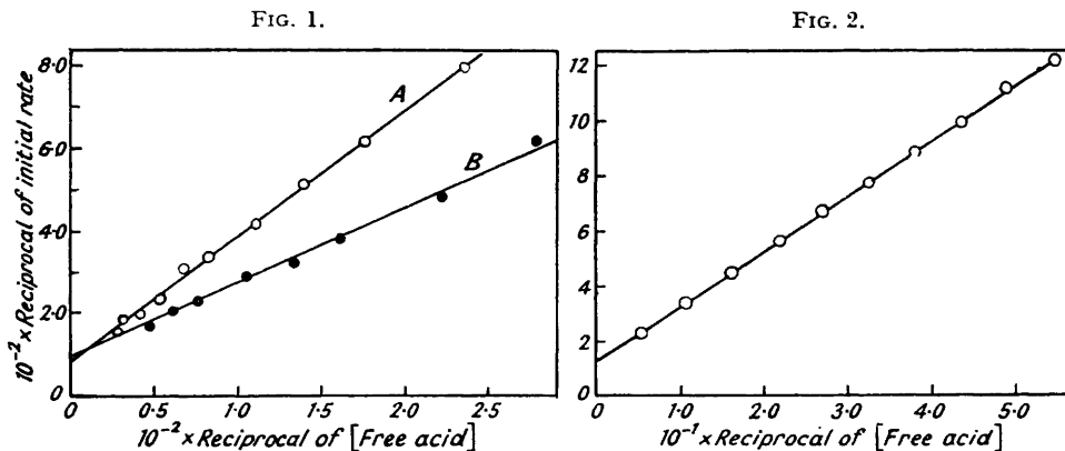
FIG. 1. Oxidations of (+)- and of meso-tartaric acid.
