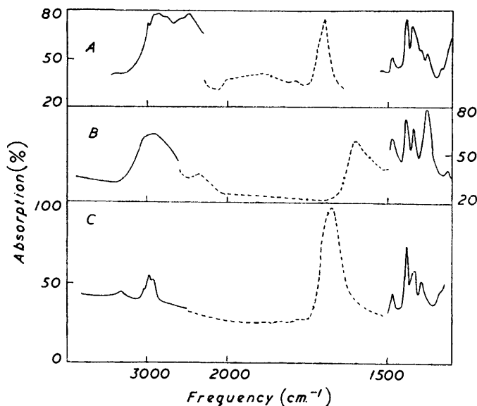
FIG. 2. Corresponding regions of the infrared spectra of solid suspensions, at arbitrary concentrations, in Nujol (-----) and hexachlorobutadiene (—), of: (A) Di(carboxymethyl)phenyl-arsine oxide (XIV; n = 1). (B) 2-Carboxyethyldiphenyl-arsine hydroxide betaine (XV). (C) Di-(2-carboxyethyl)phenyl-arsine dihydroxide dilactone (XVI; R = H).
