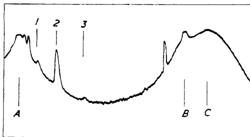
FIG. 2. Raman spectrum of the hyponitrite ion. (The Raman frequency 1383 \text{cm}^{-1} occurs twice, excited strongly by Hg \lambda 4047 Å and weakly by Hg \lambda 4078 Å.)
