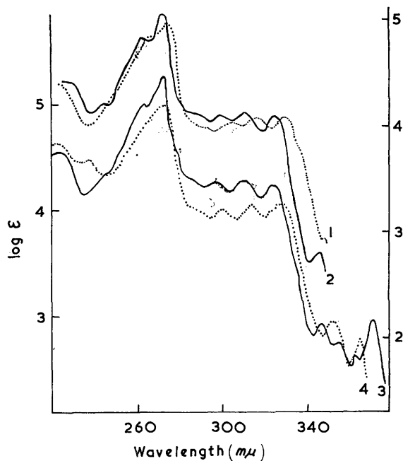
1, 3,4-Dimethylchrysen. 2, 1,2-Dimethylchrysen. 3, 2,12-Dimethylchrysen. 4, 3,5-Dimethylchrysen. Curves 1 and 2—right-hand scale.
