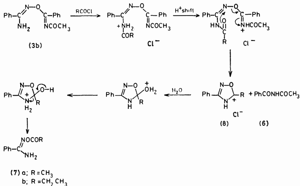
SCHEME 2 Mechanism for reaction of derivative (3b) with acyl chlorides
