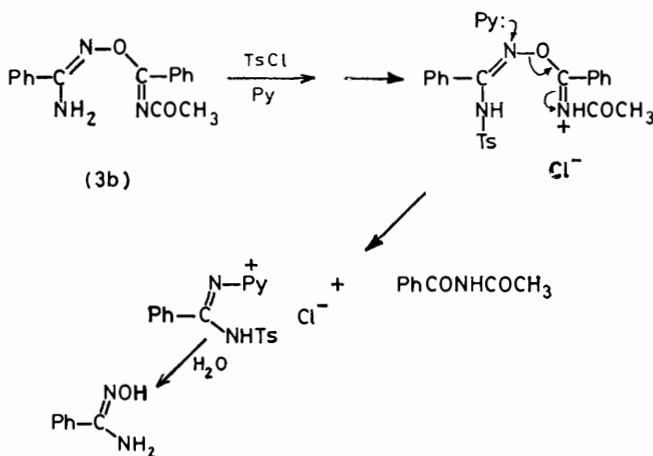
SCHEME 3 Mechanism for reaction of derivative (3b) with toluene- p -sulphonyl chloride in pyridine
