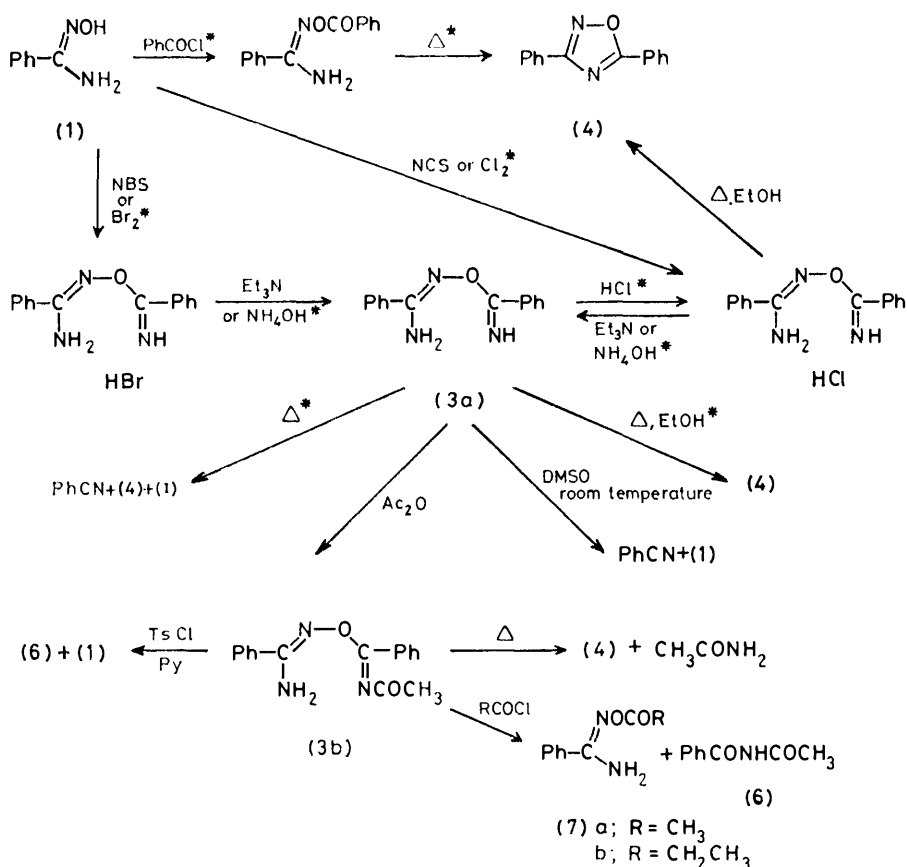
SCHEME 1 Summary of reactions reported in this paper and (*) by other authors 3,4
