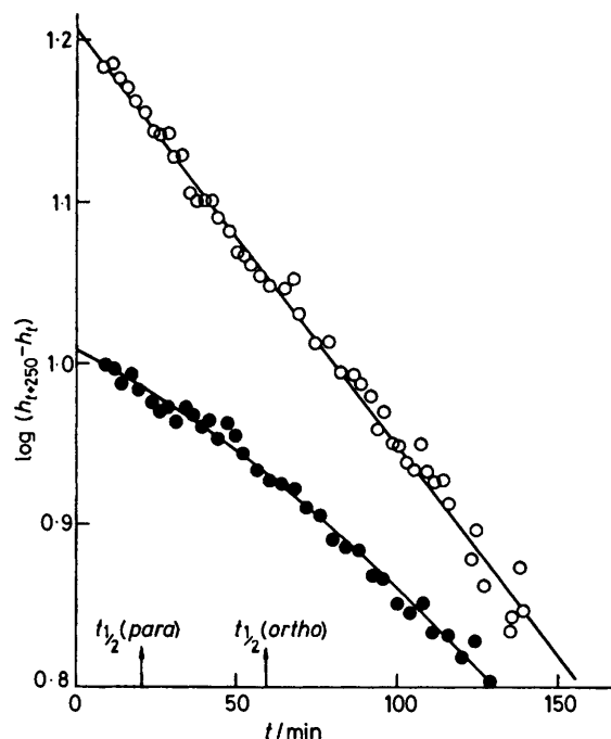
FIGURE 2 Guggenheim plots showing the effect of ring deuteration on the kinetic form of N-N hydrogen isotope exchange in 96.01% \text{D}_2\text{SO}_4 . The half-lives for exchange in the aromatic ring are also shown. 3,5\text{-Me}_2\text{C}_6\text{D}_3\text{N}^+\text{Me}_2\text{H} , \circ ; 3,5\text{-Me}_2\text{C}_6\text{H}_3\text{N}^+\text{Me}_2\text{H} , \bullet
