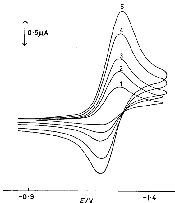
FIGURE 4 2.56 \times 10^{-3} mol dm^{-3} solution of cation (II) in DMF containing 0.05 mol dm^{-3} TPAP. Potential scans at platinum microelectrode versus Ag-AgCl-Cl - (aqueous) reference electrode. Uncorrected for iR drop or charging current; cathodic followed by anodic sweep in each case. 1, 30 mV s^{-1} ; 2, 60 mV s^{-1} ; 3, 100 mV s^{-1} ; 4, 200 mV s^{-1} ; 5, 300 mV s^{-1}
