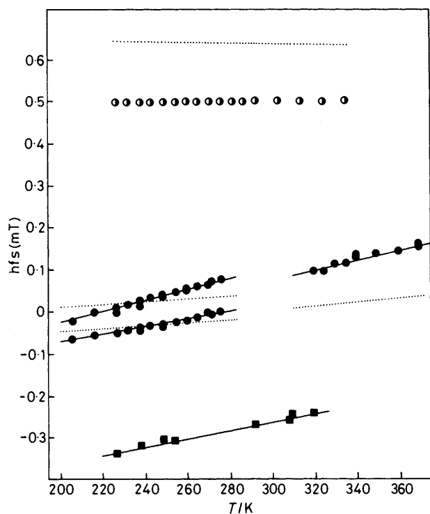
Figure 4. Temperature variation of the h.f.s. of aminopropynyl radicals (2a) and aminocyanomethyl radicals (6). Half-filled circles, experimental h.f.s. of nitrogen atom of (2a); filled circles, experimental h.f.s. of amino hydrogens of (2a); filled squares, experimental h.f.s. of amino hydrogens of (6); full lines calculated from equation (3) (see text); dotted lines, INDO calculations
