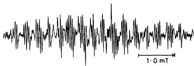
Figure 1. 9.4 GHz e.s.r. spectrum of aminoallyl radicals (1a) in neat di-t-butyl peroxide at 240 K
