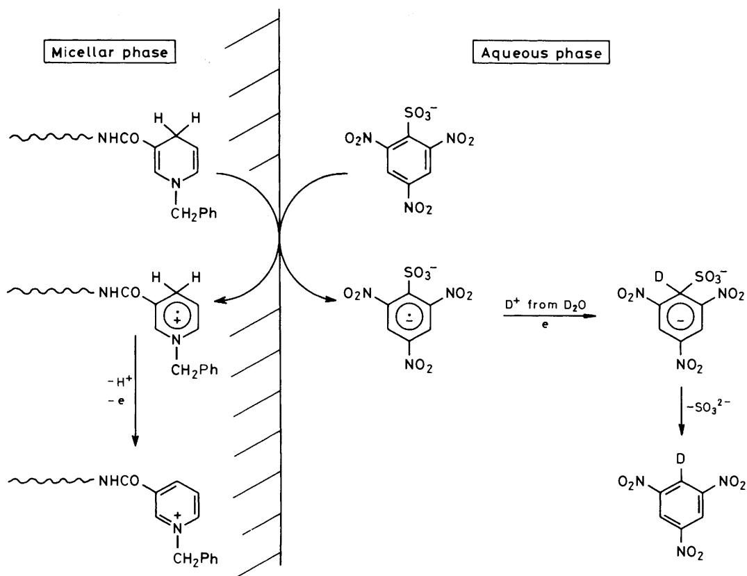
Figure 1. Schematic representation of the charge separation of a radical ion-pair formed from N -DodBzlNAH and TNBS
