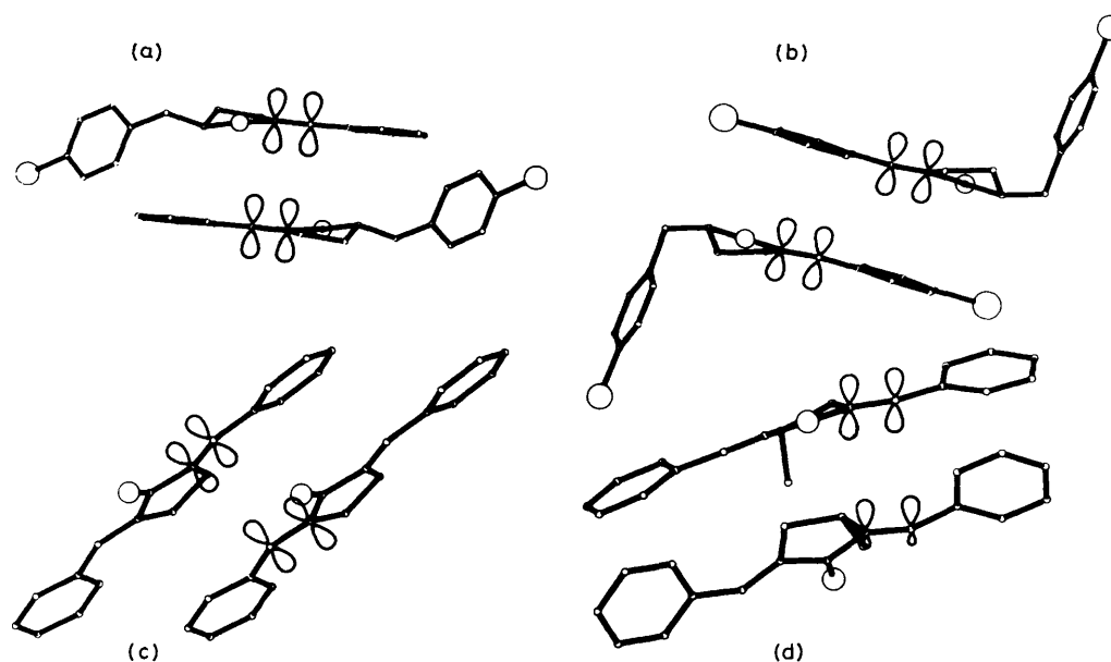
Figure 4. Illustration of different kinds of disposition of reacting double bonds in adjacent molecules in crystals of BBCP, DBCP, and some of their derivatives. These dispositions and the relevant separation distances are the principal determination of photoreactivity. (a) Double bonds in adjacent molecules are parallel and separated by ca. 4 Å in crystals of 2- p -chlorobenzyl-5-benzylidene-cyclopentanone. This crystalline solid is photoreactive. (b) Double bonds are parallel but quite far apart ( ca. 4.7 Å) in crystals of 2- p -chlorobenzyl-5- p -bromobenzylidene-cyclopentanone. This solid is photostable. (c) Double bonds are not parallel, but the planes of the benzylidene groups are, and the separation distance is only ca. 3.7 Å in DBCP. This solid is photoreactive. (d) Neither the double bonds nor the planes of the benzylidene groups are parallel in DB(+) 3 MeCP; the molecular planes are almost perpendicular to one another, despite the short separation distance ( ca. 3.9 Å) this crystalline solid is photostable
