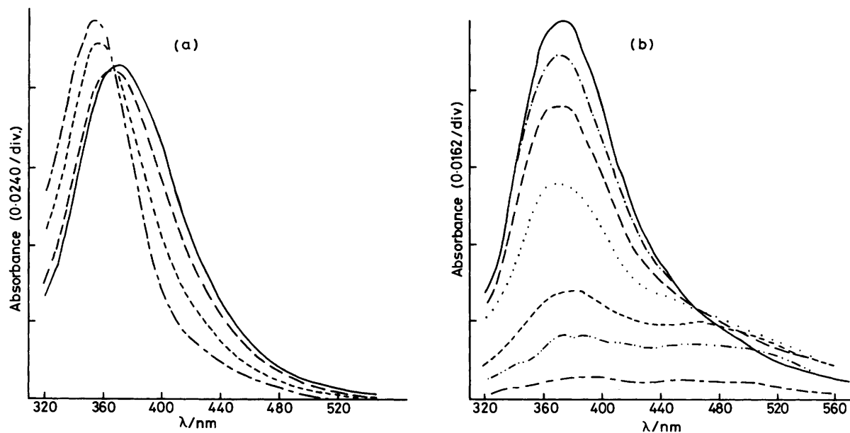
Figure 3. Time-resolved spectra of N_2O -saturated 0.1M-potassium iodide solution at pH 5.8 (a) without cysteine, 10 Gy pulse; (b) plus 5 \times 10^{-3}M cysteine, 9 Gy pulse
