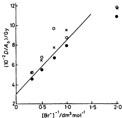
Figure 2. Plot of dose/(absorbance at discontinuity) against (bromide concentration) -1 : O, highest gun filament current (ca. 30 Gy); ×, middle gun filament current (ca. 15 Gy); ●, lowest gun filament current (ca. 7 Gy)
