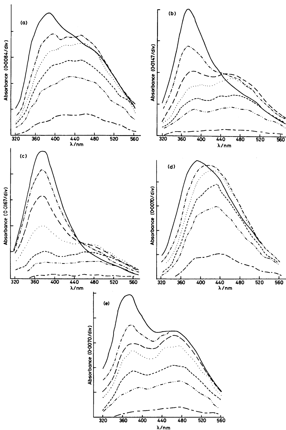
Figure 6. Time-resolved spectra of N_2O -saturated solutions of potassium iodide and cysteine at pH 7.5: (a) 0.1M-KI, 5 \times 10^{-3} M-cysteine, 8 Gy pulse; (b) 0.1M-KI, 2 \times 10^{-3} M-cysteine, 9 Gy pulse; (c) 0.1M-KI, 5 \times 10^{-4} M-cysteine, 9 Gy pulse; (d) 0.01M-KI, 5 \times 10^{-3} M-cysteine, 8 Gy pulse; (e) 1.0M-KI, 5 \times 10^{-3} M-cysteine, 8 Gy pulse
