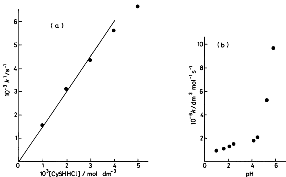
Figure 5. Kinetics of decay of I_3^- at 370 nm following 24 Gy pulse. (a) Pseudo-first-order rate constant against cysteine hydrochloride concentration at pH 2.4. (b) Second-order rate constant against pH 0.1M-potassium iodide, 2 \times 10^{-3}M -cysteine (see Discussion section)
