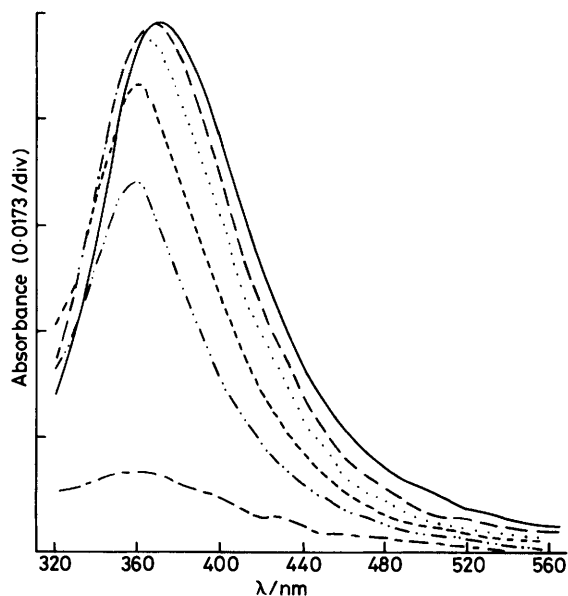
Figure 4. Time-resolved spectra of N_2O -saturated 0.1M-potassium iodide and 5 \times 10^{-3}M cysteine hydrochloride at pH 2.35, 9 Gy pulse
