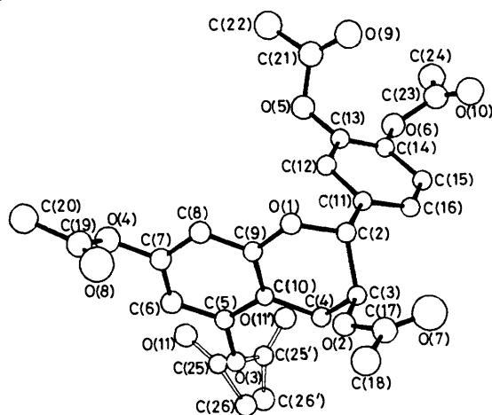
Figure 2. Conformation of penta- O -acetyl-(+)-catechin in the crystal
