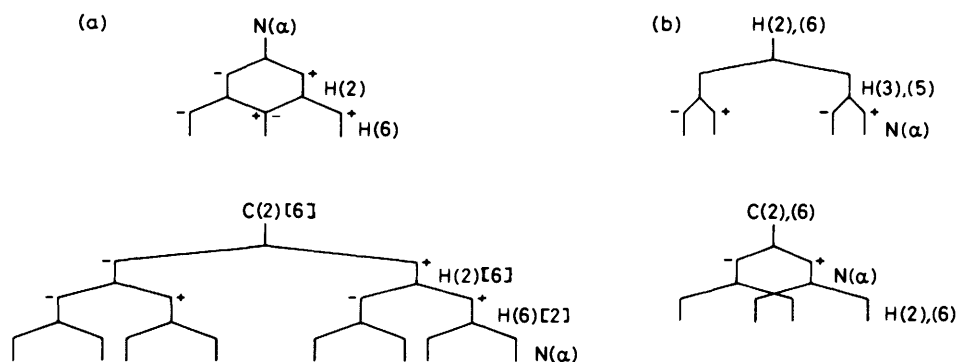
Figure 7. (a) Schematic diagrams for \text{N}(\alpha) and \text{C}(2),(6) at a proton-coupled state. (b) Schematic diagrams for \text{H}(2),(6) and \text{C}(2),(6) . In \text{C}(2),(6) , residual J'(\text{C-H}) splittings of ^1J[\text{C}(2),(6)\text{-H}(2),(6)] are shown; the other couplings, e.g. ^2J[\text{C}(2)\text{-H}(3)] , ^3J[\text{C}(2)\text{-H}(6)] , and ^4J[\text{C}(2)\text{-H}(5)] , are not shown here, because they are fully decoupled at the irradiation power used. ^1J[\text{C}(2),(6)\text{-H}(2),(6)] = 160.8 \pm 0.3 Hz, ^3J[\text{C}(2)\text{-H}(6)] [ ^3J[\text{C}(6)\text{-H}(2)] ] = 5.8 \pm 0.3 Hz, ^2J[\text{C}(2),(6)\text{-N}(\alpha)] = 4.3 \pm 0.3 Hz, ^3J[\text{N}(\alpha)\text{-H}(2),(6)] = 1.5 \pm 0.2 Hz, ^3J[\text{H}(2)\text{-H}(3)] [ ^3J[\text{H}(5)\text{-H}(6)] ] = 8.8 \pm 0.2 Hz, and J'(\text{C-H}) = 7\text{--}8 Hz
