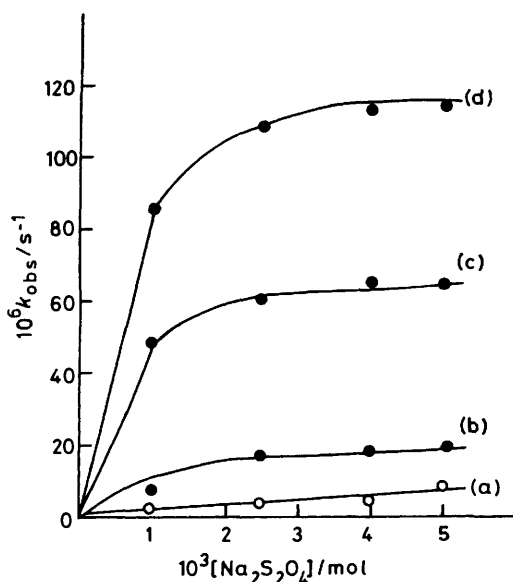
Figure 3. Effect of concentration of Na 2 S 2 O 4 in 5 ml of the outer aqueous phase on k obs. values for debromination of 1,2-dibromo-1,2-diphenylethane at 30 °C. [1,2-Dibromo-1,2-diphenylethane] 1.0 × 10 -7 mol in 10 μl of the inner chloroform solution, [viologen] (5–6) × 10 -8 mol [(26–28) μg of poly(C n V 2+ )] per capsule. (a) Non-grafted capsule, (b) poly(C 3 V 2+ )-grafted capsule, (c) poly(C 6 V 2+ )-grafted capsule, (d) poly(C 10 V 2+ )-grafted capsule
