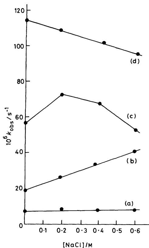
Figure 5. Effect of ionic strength on k_{obs} values of debromination of 1,2-dibromo-1,2-diphenylethane at 30 °C. [1,2-Dibromo-1,2-diphenylethane] 1.0 \times 10^{-7} mol in 10 \mu l of the inner chloroform solution, [Na_2S_2O_4] 5.0 \times 10^{-3} mol in 5 ml of the outer aqueous solution (pH 10), [viologen] (5-6) \times 10^{-8} mol [(26-28) \mu g of poly( C_nV^{2+} )] per capsule. (a) Non-grafted capsule, (b) poly( C_3V^{2+} )-grafted capsule, (c) poly( C_6V^{2+} )-grafted capsule, (d) poly( C_{10}V^{2+} )-grafted capsule
