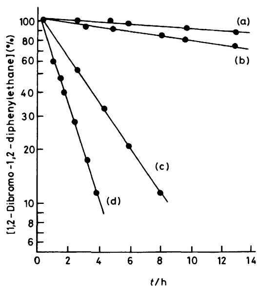
Figure 2. Plots of percentage 1,2-dibromo-1,2-diphenylethane in the inner chloroform solution as a function of time at 30 °C. [1,2-Dibromo-1,2-diphenylethane] 1.0 \times 10^{-7} mol in 10 \mu l of the inner chloroform solution, [ Na_2S_2O_4 ] 5.0 \times 10^{-3} mol in 5 ml of the outer aqueous solution (pH 10), [viologen] (5-6) \times 10^{-8} mol [26–28 \mu g of poly( C_nV^{2+} )] per capsule. (a) Non-grafted capsule, (b) poly( C_3V^{2+} )-grafted capsule, (c) poly( C_6V^{2+} )-grafted capsule, (d) poly( C_{10}V^{2+} )-grafted capsule
