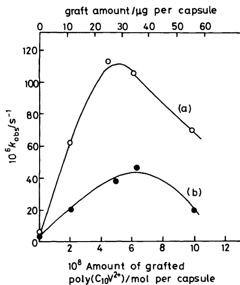
Figure 4. Effect of graft amount of poly( C_{10}V^{2+} ) per capsule on k_{obs} values at 30 °C. [Na_2S_2O_4] 5.0 \times 10^{-3} mol in 5 ml of the outer aqueous phase (pH 10). (a) Debromination of 1,2-dibromo-1,2-diphenylethane ( 1.0 \times 10^{-7} mol), (b) reduction of azobenzene ( 1.0 \times 10^{-6} mol)
