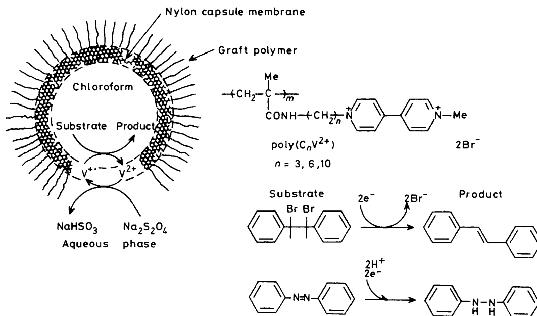
Figure 1. A capsule membrane grafted with viologen-containing polymer [poly( C_nV^{2+} ); n = 3, 6, 10 ] as a reactor for electron-transfer catalysis
