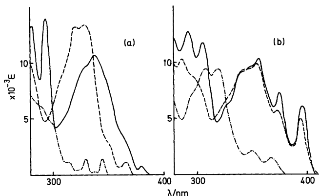
Figure. (a) Absorption spectrum of phenanthridine N -oxide in benzene (—) and in ethanol (-----) and of phenanthridine in benzene (---); (b) Absorption spectrum of 6-cyanophenanthridine N -oxide in benzene (—) and in ethanol (-----) and of 6-cyanophenanthridine in benzene (---)
