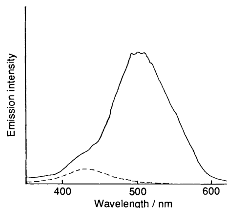
Figure 5. Emission spectrum of compound (1a) adsorbed on clay (—) and without clay (---). Excited at 330 \text{ nm} for 10 \text{ } \mu\text{mol dm}^{-3} each of compound (1a) and clay in water containing 0.02% methanol. The emission maxima of substituted stilbazolium ions are shown in Table 3.
