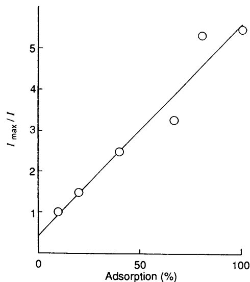
Figure 7. Dependence of the excimer fluorescence intensity ( I ) of compound (1a) upon its degree of adsorption; see Figure 6 for conditions. I_{\text{max}} is the maximum intensity of excimer fluorescence at 10% adsorption.
