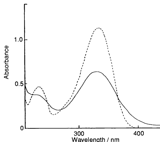
Figure 4. Absorption spectrum of compound (1a) adsorbed on Saponite clay (—) in water; 50 \text{ } \mu\text{mol dm}^{-3} (1a), 50 \text{ } \mu\text{mol dm}^{-3} equivalent clay, and 60 \text{ } \mu\text{mol dm}^{-3} HCl. The dotted line (---) is the absorption of compound (1a) in homogeneous aq. solution; 50 \text{ } \mu\text{mol dm}^{-3} (1a) and 60 \text{ } \mu\text{mol dm}^{-3} HCl.
