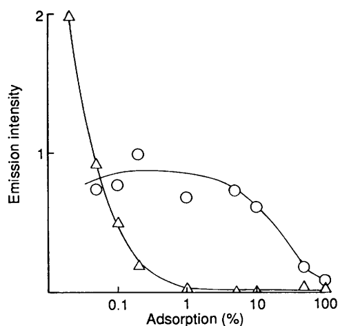
Figure 6. Dependence of emission intensity upon the degree of adsorption of compound (1a) on clay interlayer: 1 \mu\text{mol dm}^{-3} (1a), 1–5 000 \mu\text{mol dm}^{-3} clay, and 1.2 \mu\text{mol dm}^{-3} HCl. Excitation at 335 nm; emission of monomer ( \Delta ) and excimer ( \circ ). Degree of adsorption was calculated from the ratio of (1a) vs. CEC of clay.
