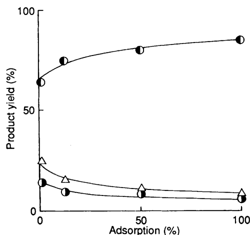
Figure 3. Effect of degree of adsorption of substrate (1a) on the efficiency of photodimerization; \bullet , yield of (2a); \circ , yield of (3a); \triangle , yield of (Z)-(1a). A suspended solution of compound (1a) ( 1 \text{ mmol dm}^{-3} ) and clay ( 1\text{--}80 \text{ mmol dm}^{-3} ) was irradiated at >300 \text{ nm} for 30 min under argon. The degree of adsorption was calculated from the ratios of (1a) vs. the CEC of clay.
