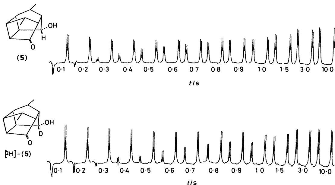
Figure 3. Spin saturation transfer between methyl groups in the ^1\text{H} NMR spectra of (5) and [\text{2H}] -(5) in \text{CF}_3\text{SO}_3\text{H}-\text{SO}_2 solution.
