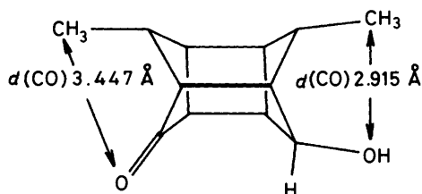
Figure 1. Stereochemical relationship of methyl groups and oxygens in (5).
