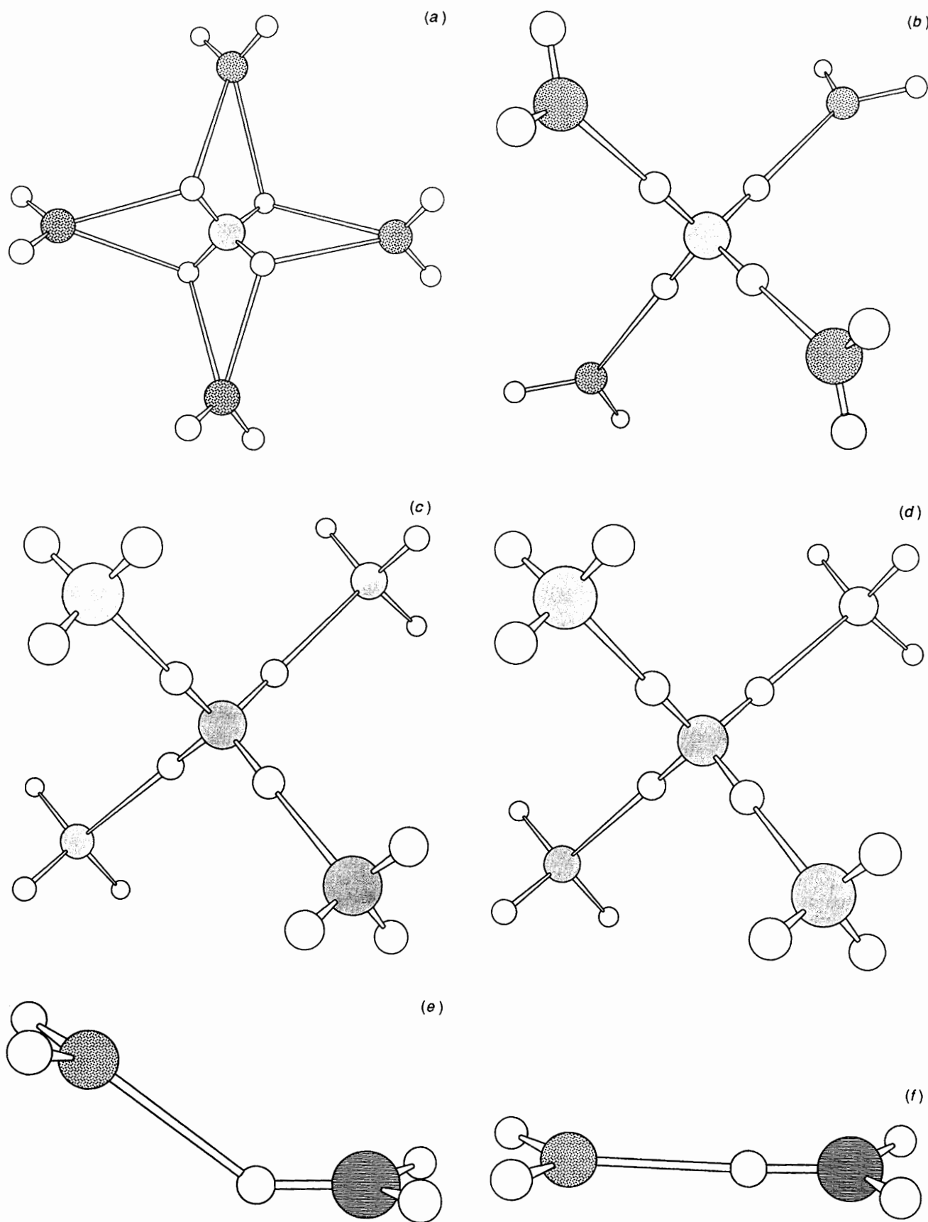
Figure 1. (a) AM1 and (b) PM3 calculated structures for the hydrogen-bonded complexes \text{NH}_4^+ \cdot 4\text{H}_2\text{O} ; (c) and (d) for \text{NH}_4^+ \cdot 4\text{NH}_3 ; (e) and (f) for \text{NH}_3^{++} \cdot \text{H}_2\text{O} ; (g) and (h) for \text{O}_2^{--} \cdot 2\text{H}_2\text{O} ; (i) and (j) for \text{HO}^- \cdot 4\text{H}_2\text{O} .
