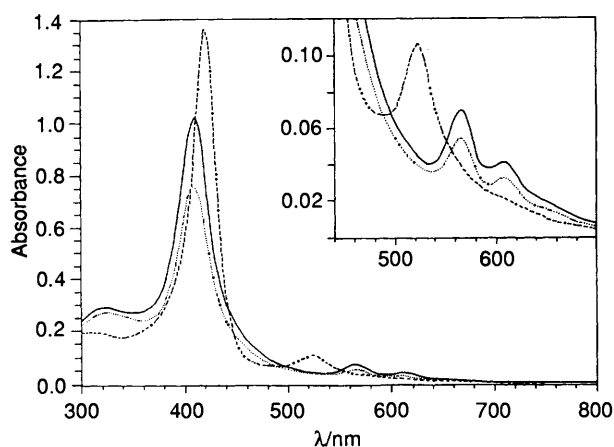
Fig. 4 UV-VIS spectra of Fe III TSP (8.0 \times 10^{-6} mol dm ^{-3} ) in borate buffer solution (0.1 mol dm ^{-3} , pH 9.2) before (—), 30 s (---) and 60 min (···) after the addition of 5 mol equiv. of MPS
