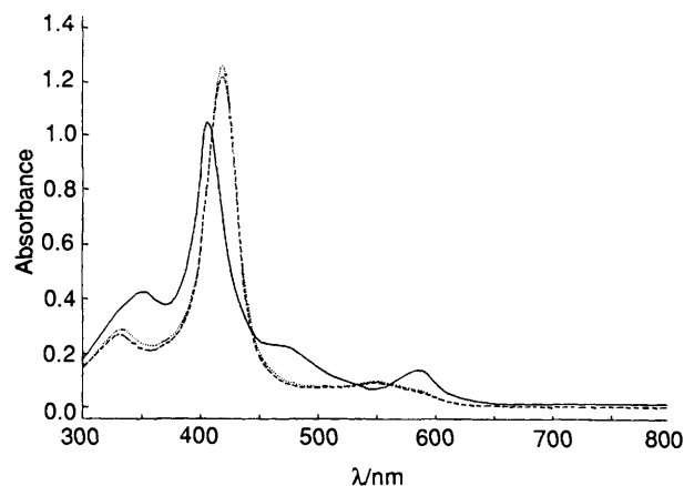
Fig. 3 UV-VIS spectra of Fe III T2MPyP (9.07 × 10 -6 mol dm -3 ) in borate buffer (0.1 mol dm -3 , pH 9.2) before (—) and after addition of 3 mol equiv. of Bu t O 2 H (···) or MPS (----)
