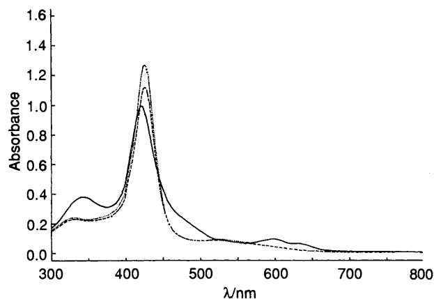
Fig. 1 UV-VIS spectra of Fe III T4MPyP ( 9.41 \times 10^{-6} mol dm -3 ) in borate buffer (0.1 mol dm -3 , pH 9.2) before (—) and after addition of 3 mol equiv. of Bu'O 2 H (····) or MPS (----)
