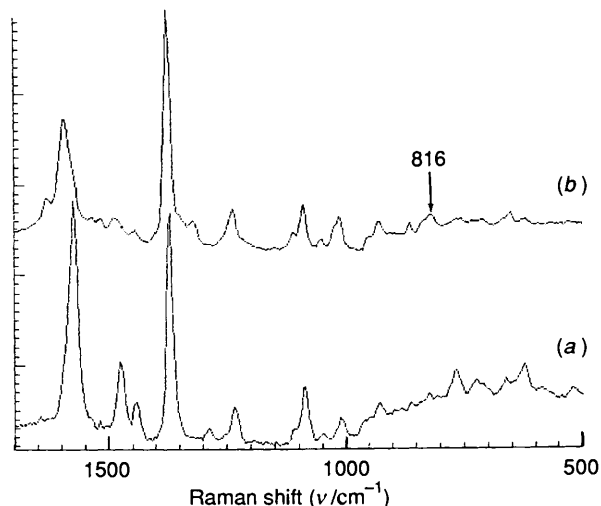
Fig. 9 Resonance Raman spectrum of \text{Fe}^{\text{III}}\text{TDCSPP} in borate buffer ( 0.1 mol \text{dm}^{-3} , pH 9.2) before (a) and after (b) the addition of 3 mol equiv. of \text{Bu}'\text{O}_2\text{H}
