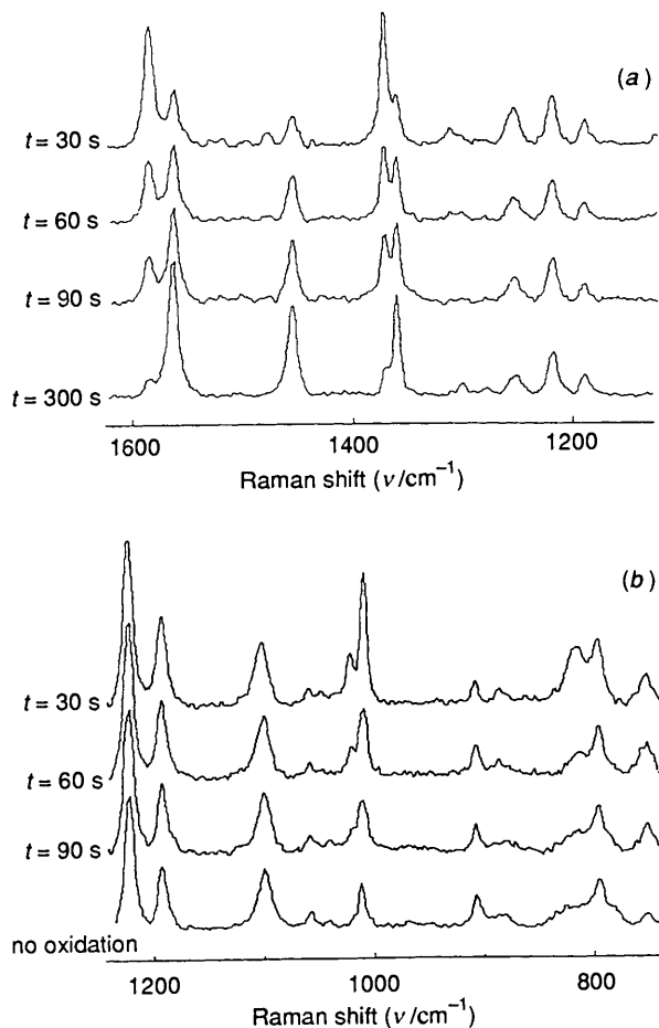
Fig. 8 Time-resolved resonance Raman spectra of \text{Fe}^{\text{III}}\text{T4MPyP} ( 10^{-4} mol \text{dm}^{-3} ) in aqueous solution following the addition of 3 mol equiv. of \text{Bu}'\text{O}_2\text{H} . (a) High-frequency spectrum (pH 9.2); (b) low-frequency spectrum (pH 9.4).
