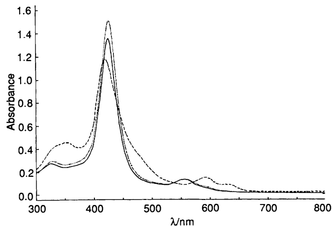
Fig. 5 UV-VIS spectra of Fe III T4MPyP (1.35 \times 10^{-5} mol dm ^{-3} ) in methanol before (---) and after the addition of 100 mol equiv. of Bu t O 2 H (···) or 40 mol equiv. of 3-CPBA (—)
