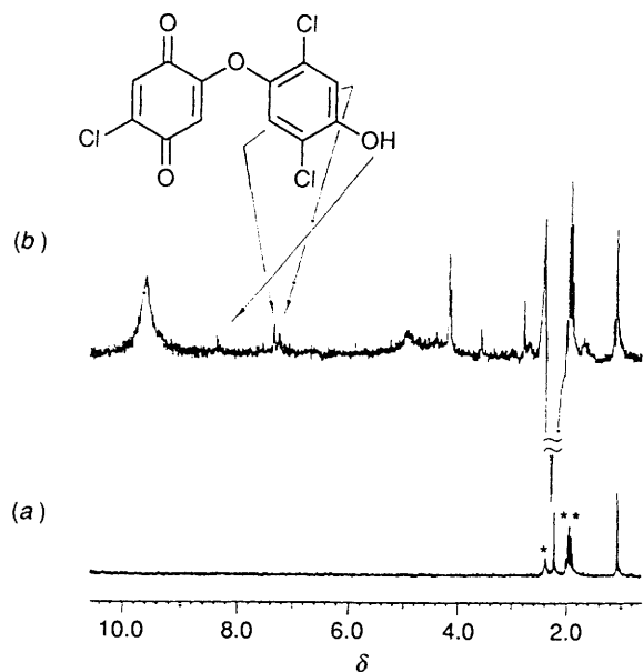
Fig. 1 ^1\text{H} NMR spectra of 1a ( 0.02 \text{ mol dm}^{-3} ) in the presence of 2a ( 0.04 \text{ mol dm}^{-3} ) in [\text{D}_3\text{H}_3]\text{acetonitrile} . (a) Dark, (b) light. * \text{H}_2\text{O} (solvent impurity), ** \text{CHD}_2\text{CN} (solvent impurity).
