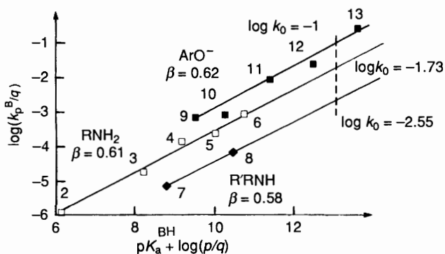
Fig. 3 Statistically-corrected Brønsted plots for the deprotonation of 3 by phenoxide and amine bases in \text{H}_2\text{O}-\text{Me}_2\text{SO} (20:80); T = 25^\circ\text{C} , I = 0.5 \text{ mol dm}^{-3} \text{ NMe}_4\text{Cl} . The numbering of the catalysts is indicated in Table 1.
