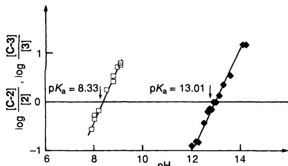
Fig. 1 The variation of the ratio of ionized to non-ionized triphenylmethanes 2 ( pK_a = 8.33 ) and 3 ( pK_a = 13.01 ) as a function of pH in H_2O-Me_2SO (20:80); T = 25^\circ C ; I = 0.5 \text{ mol dm}^{-3} NMe_4Cl
