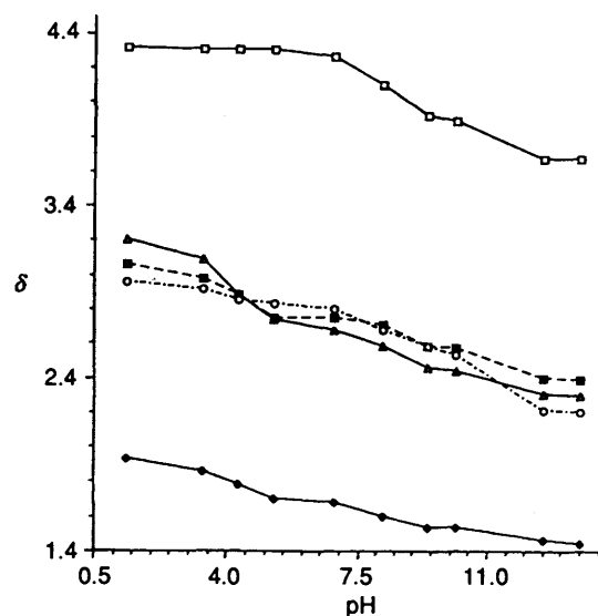
Fig. 2 Plot of the 1 H NMR chemical shifts of the ligand 4 vs. pH. □, H-1,14; ■, H-5,10; △, H-7,8; ○, H-3,12; ◆, H-4,11.
