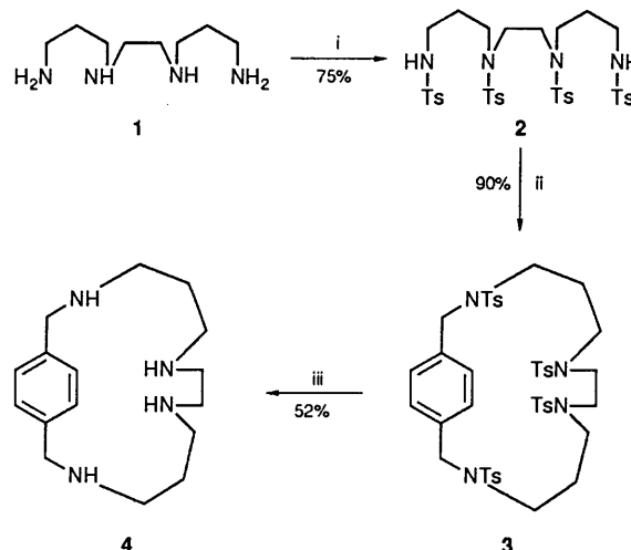
Scheme 1 Reagents and conditions: i, TsCl, NaOH; H 2 O/THF; ii, \alpha , \alpha' -dibromo- p -xylene, K 2 CO 3 , CH 3 CN; iii, HBr/AcOH 33%, PhOH
