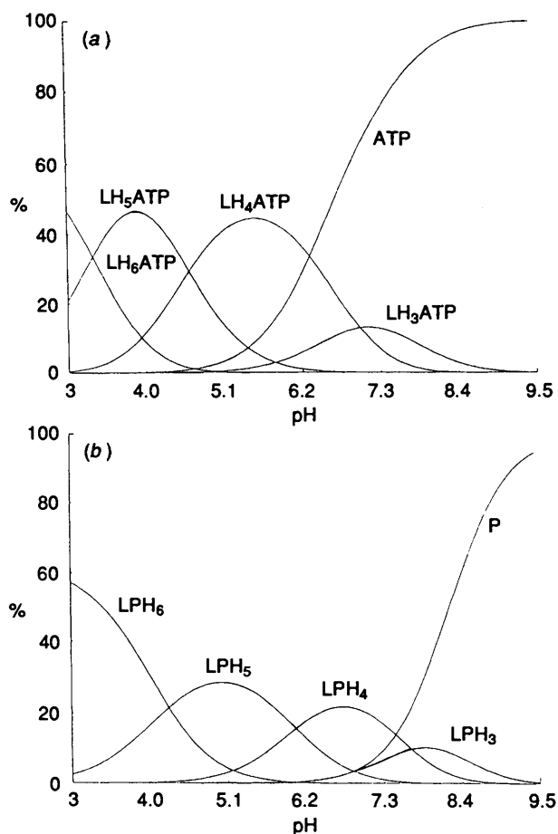
Fig. 7 Distribution diagrams of the species in equilibria for the system A-4. Charges have been omitted for clarity. [A] = [4] = 10 -3 mol dm -3 . (a) A = ATP. (b) A = pyrophosphate.
