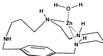
Fig. 6 Possible model for tricoordinate interaction between 4 and \text{Zn}^{2+}
