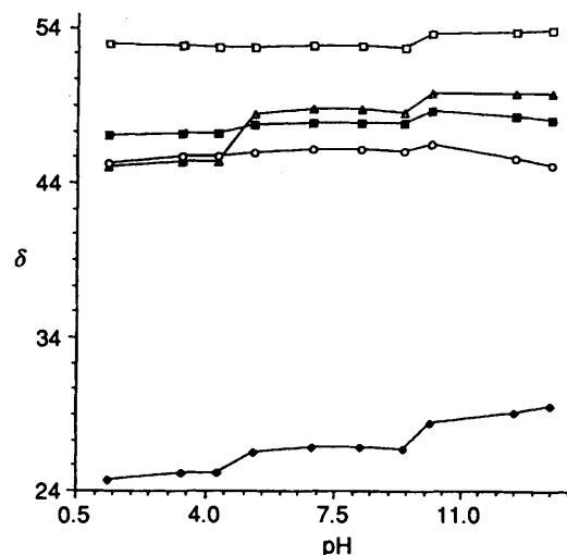
Fig. 3 Plot of the 13 C NMR chemical shifts for the aliphatic carbon atoms of the ligand 4 vs. pH. □, C-1,14; ■, C-5,10; △, C-7,8; ○, C-3,12; ◆, C-4,11.
