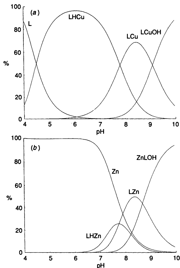
Fig. 5 Distribution diagrams of the species in equilibria for the system \text{M}^{2+} - 4 . Charges have been omitted for clarity. [\text{M}] = [\text{4}] = 10^{-3} \text{ mol dm}^{-3} . (a) \text{M} = \text{Cu} . (b) \text{M} = \text{Zn} .
