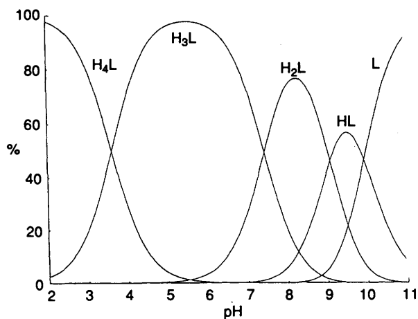
Fig. 1 Distribution diagram of the species in equilibrium for the system H + - 4 . Charges have been omitted for clarity.
