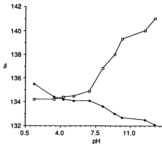
Fig. 4 Plot of the ^{13}\text{C} NMR chemical shifts for the aromatic carbon atoms of the ligand 4 vs. pH. \square , C-15,18; \blacklozenge , C-16,17,19,20.
