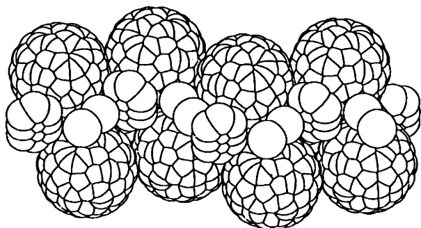
Fig. 3 Repeating units of C_{60}I_2 -toluene leading to a staggered network of both C_{60} and iodine molecules within the crystal lattice
