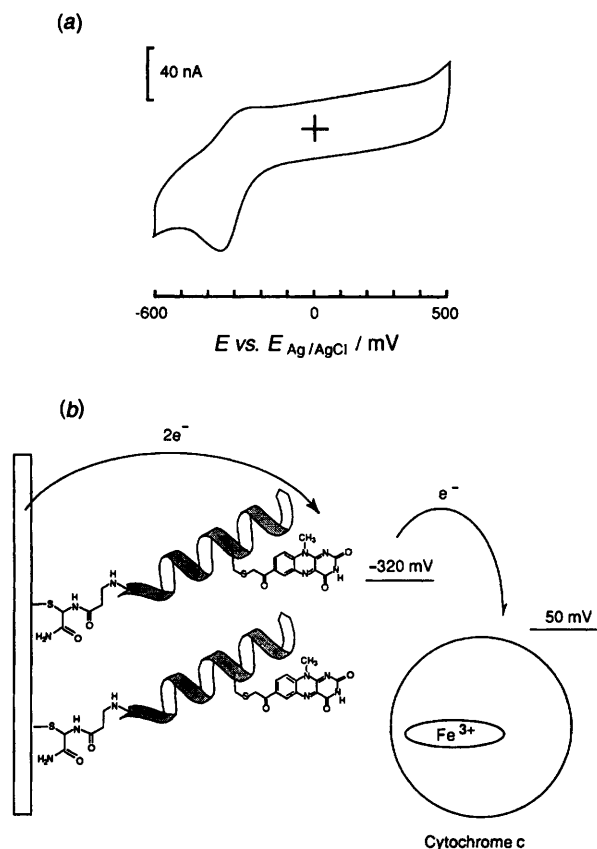
Fig. 7 (a) Cyclic voltammogram for the gold electrode modified with the Fla 8 -1 \alpha -SH in 5.0 \times 10^{-5} \text{ mol dm}^{-3} cytochrome c- 0.1 \text{ mol dm}^{-3} phosphate buffer, pH 7.0 at 25^\circ\text{C} ; the sweep rate was 10 \text{ mV s}^{-1} . (b) Illustration of the electron transfer from the electrode to cytochrome c mediated by Fla-1 \alpha -SH bound on the gold surface.
