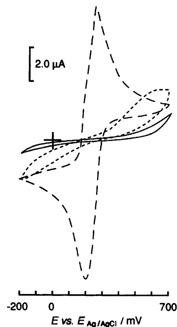
Fig. 3 Cyclic voltammograms for Fla 6 -1 \alpha -SH-modified gold electrode prepared in aqueous solution (—), Fla 6 -1 \alpha -SH modified gold electrode prepared in TFE solution (----) and bare gold (unmodified) electrode (-·-·-). Measured in 2.0 \times 10^{-3} mol dm -3 K 3 [Fe(CN) 6 ]-0.1 mol dm -3 phosphate buffer, pH 7.0 at 100 mV s -1 sweep rate at 25 °C.
