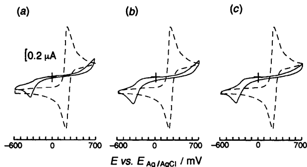
Fig. 6 Cyclic voltammograms for the gold electrodes modified with the flavin-conjugated peptides (—) and bare gold (unmodified) electrode (---) in 2.0 \times 10^{-3} \text{ mol dm}^{-3} \text{K}_3[\text{Fe}(\text{CN})_6] - 0.1 \text{ mol dm}^{-3} phosphate buffer, pH 7.0 at 25^\circ\text{C} ; (a) Fla 6 -1 \alpha -SH, (b) Fla 7 -1 \alpha -SH, (c) Fla 8 -1 \alpha -SH. The sweep rate was 100 \text{ mV s}^{-1} .
