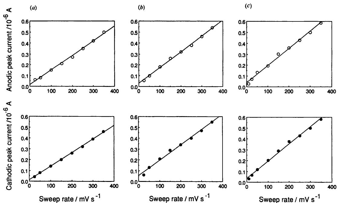
Fig. 5 Plots of anodic and cathodic peak currents as a function of the sweep rate for Fla-peptide modified electrodes in 0.1 mol dm -3 phosphate buffer, pH 7.0 at 25 °C; (a) Fla 6 -1α-SH, (b) Fla 7 -1α-SH, (c) Fla 8 -1α-SH
