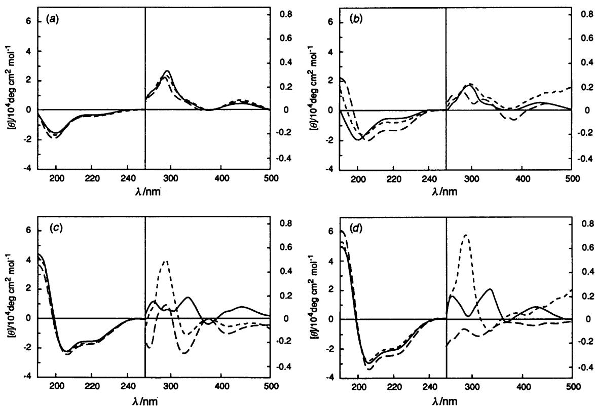
Fig. 2 CD spectra of Fla-1 \alpha - [(a) and (b)] and Fla-2 \alpha -peptides [(c) and (d)] in 2.0 \times 10^{-2} mol dm -3 Tris·HCl buffer, pH 7.4 [(a) and (c)] and TFE [(b) and (d)]. (—) Fla 6 -1 \alpha and 2 \alpha peptides; (----) Fla 7 -1 \alpha and 2 \alpha peptides; (- - -) Fla 8 -1 \alpha and 2 \alpha peptides. [\theta] at the amide region is the mean residual weight ellipticity, and [\theta] at the flavin absorption region is the molar ellipticity for Fla. [Fla-1 \alpha ] = 2.0 \times 10^{-5} mol dm -3 , [Fla-2 \alpha ] = 1.0 \times 10^{-5} mol dm -3 ; 25 °C.
