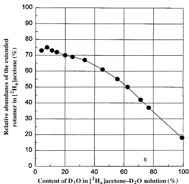
Fig. 5 Effect of D 2 O concentration on the relative proportions of the extended and compact rotamer of 1
