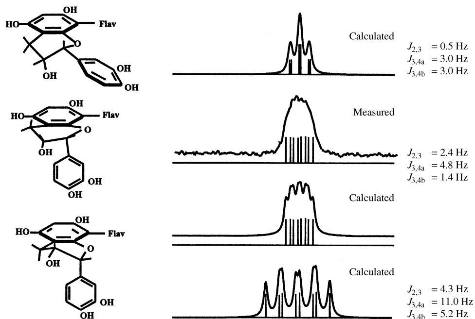
Fig. 6 PCPMR lineshape analyses of the H-3 F proton in 1 when recorded in D 2 O
