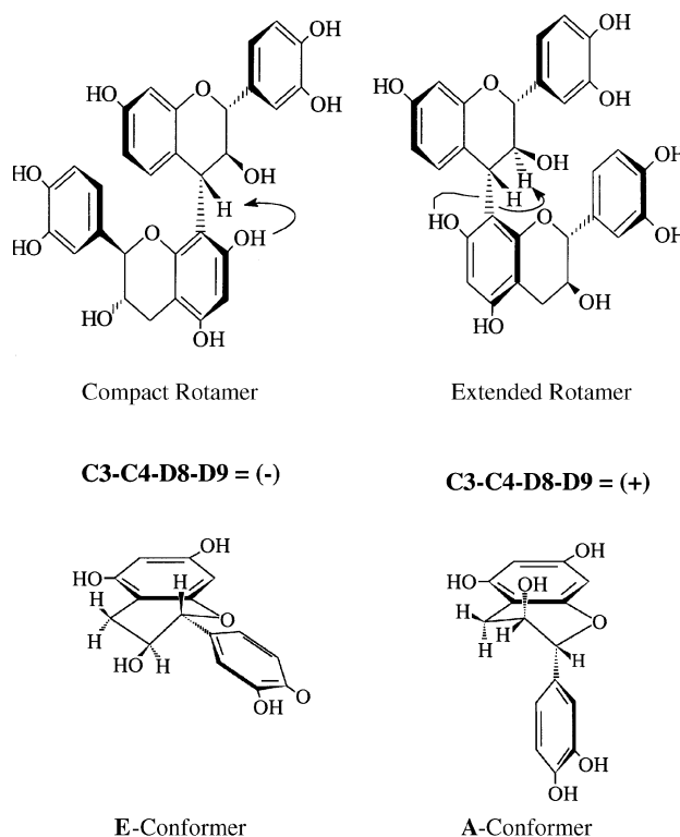
Fig. 1 Examples representing rotational and heterocyclic ring conformational heterogeneity in dimeric procyanidins. Arrows indicate observed NOE in proflisetinidin analogues. 6
