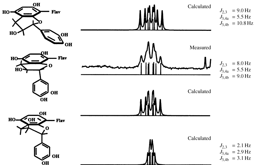
Fig. 8 PCPMR lineshape analyses of the H-3 F proton in 2 when recorded in D 2 O.
