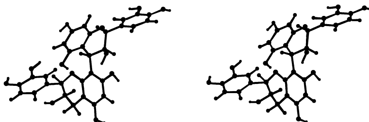
Fig. 3 Stereoview of the extended rotamer of 1
