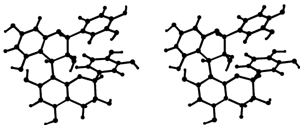
Fig. 7 Stereoview of the compact rotamer of 1
