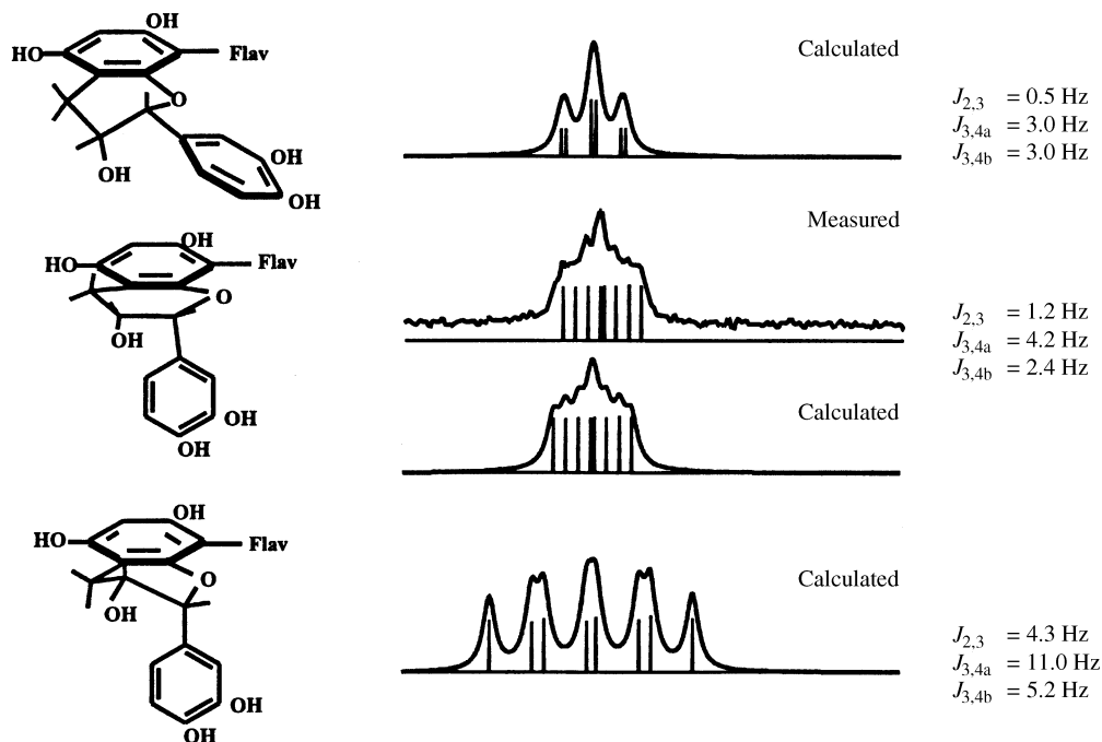
Fig. 4 PCPMR lineshape analyses of the H-3 F proton in 1 when recorded in [ 2 H 6 ]acetone with a small amount of D 2 O
