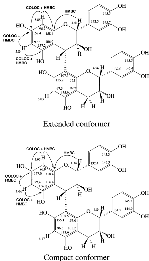
Fig. 2 HMBC correlations used to assign H-6 A and H-8 A in 1
