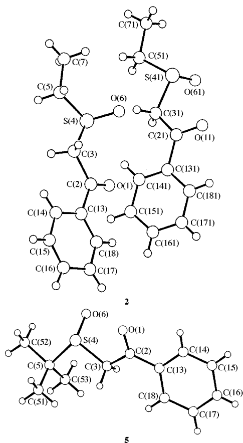
Fig. 2 X-Ray crystal structures of compounds 2 and 5 with heavy atoms labelling. The size of the atoms is arbitrary. For 2 the two independent molecules present in the unit cell are reported.
