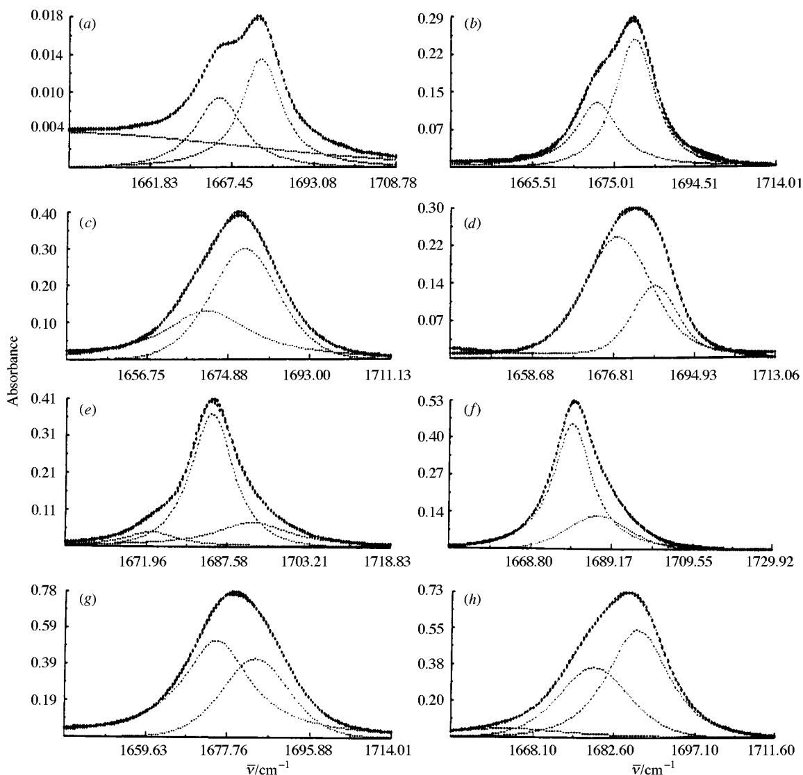
Fig. 1 IR analytically resolved carbonyl stretching bands of the \alpha -methylsulfinylacetophenone 1 and of \alpha - tert -butylsulfinylacetophenone 5 : in n -hexane (a), (e); carbon tetrachloride (b), (f); chloroform (c), (g); and acetonitrile (d), (h), respectively
