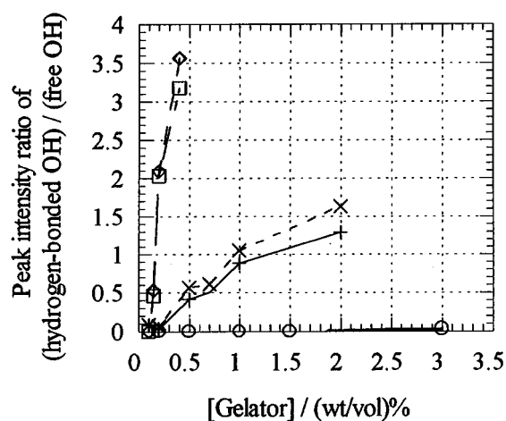
Fig. 3 Plots of the peak intensity ratio of (hydrogen-bonded \nu_{\text{OH}} peak) / (free \nu_{\text{OH}} peak) vs. the gelator concentration in benzene. \diamond , \nu_{\text{OH}} (3505 \text{cm}^{-1} ) / \nu_{\text{OH}} (3571 \text{cm}^{-1} ) of 2 ; \square , \nu_{\text{OH}} (3423 \text{cm}^{-1} ) / \nu_{\text{OH}} (3571 \text{cm}^{-1} ) of 2 ; \times , \nu_{\text{OH}} (3385 \text{cm}^{-1} ) / \nu_{\text{OH}} (3576 \text{cm}^{-1} ) of 1 ; + , \nu_{\text{OH}} (3302 \text{cm}^{-1} ) / \nu_{\text{OH}} (3576 \text{cm}^{-1} ) of 1 ; \circ , \nu_{\text{OH}} (3440 \text{cm}^{-1} ) / \nu_{\text{OH}} (3570 \text{cm}^{-1} ) of 3 .
