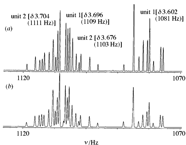
Fig. 3 ^1\text{H} NMR spectrum of 1d ; comparison of the \text{Ar}-\text{OCH}_2-\text{CH}_2-\text{OCH}(\text{i})_2\text{CH}(\text{ii})_2-\text{OCH}(\text{i})_2\text{CH}(\text{ii})_2\text{OH} , viz. units 1 and 2 [upper trace, experimental (solvent \text{C}_2\text{D}_2\text{Cl}_4 , 80 °C) and lower trace, simulated; see also Tables 5 and 8]
