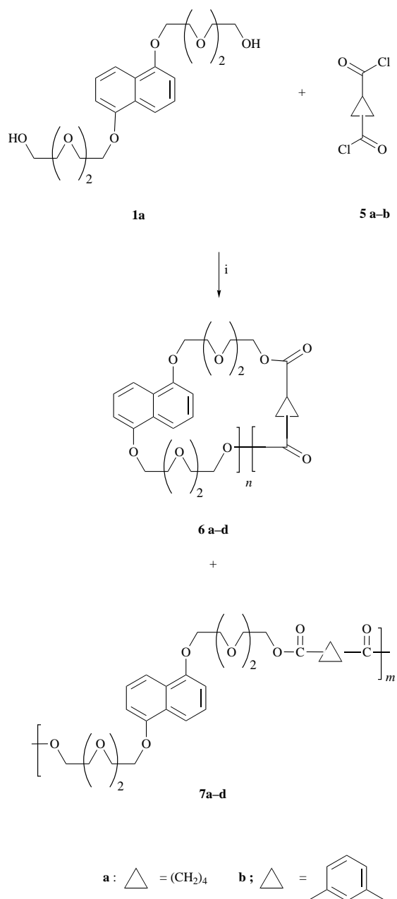
Scheme 2 Reagents and conditions: i, 1,2-dichloroethane, pyridine, reflux
