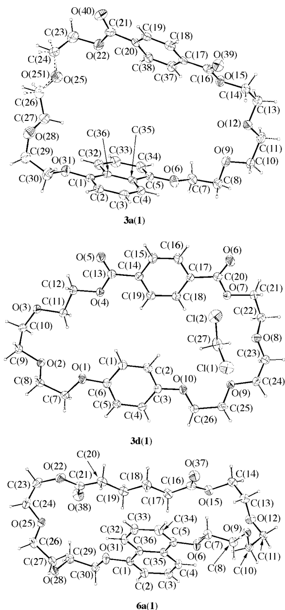
Fig. 5 ORTEP plots (50% probability) of the crownphanes 3a (1), 3d (1) and 6a (1). Atom numberings of 3a (1), 3d (1) and 6a (1) are not in agreement with IUPAC guidelines (see Experimental section).
