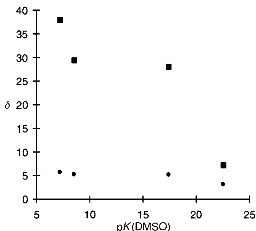
Fig. 5 ^1\text{H} (●) and ^{13}\text{C} (■) chemical shifts ( \text{R}_3\text{P}^+\text{CH}_2\text{Y} ), measured in [\text{}^2\text{H}_6]\text{DMSO} , plotted vs. \text{p}K(\text{DMSO})^1
