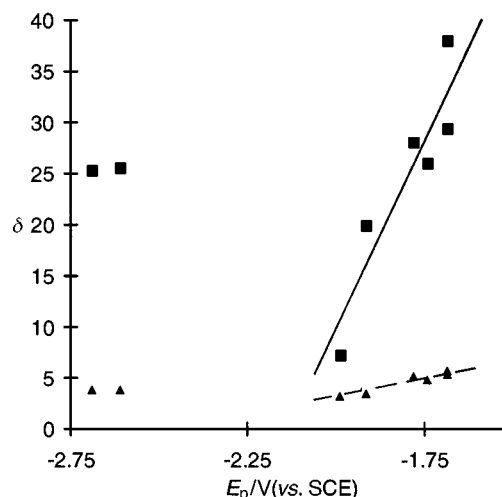
Fig. 6 ^1\text{H} (Δ) and ^{13}\text{C} (■) chemical shifts ( \text{R}_3\text{P}^+\text{CH}_2 ), measured in [\text{}^2\text{H}_6]\text{DMSO} , plotted vs. the irreversible reduction potentials for ( \text{R}_3\text{P}^+\text{CH}_2 ) (see Table 1)
