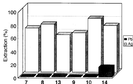
Fig. 5 Extraction (%) of Ag I and Pb II by crownophanes 7–10 , 13 and 14
