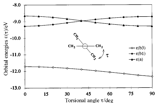
Fig. 5 Variation in energy of the \phi(a) and \phi(b_1) frontier orbitals of TME with respect to the dihedral angle, \tau . The orbital energies are from UHF/6-31+G(d) calculations on TME ^3\text{B}_1 .
