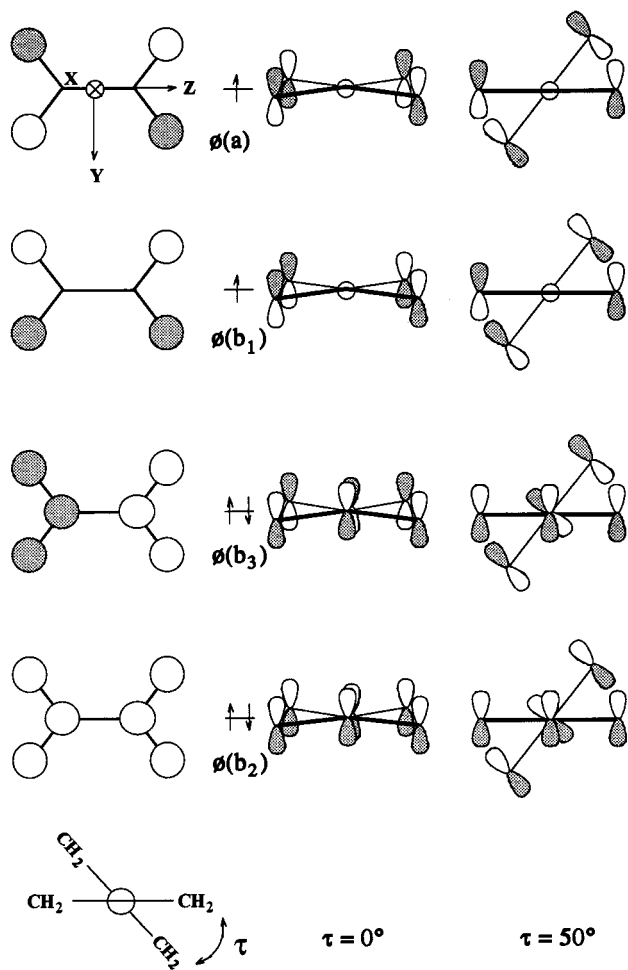
Fig. 4 Sketches of the a, b 1 , b 2 , and b 3 π orbitals of TME
