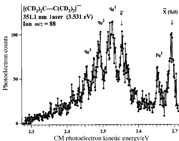
Fig. 3 A plot of the negative ion spectrum of the [(\text{CD}_2)_2\text{C}-\text{C}(\text{CD}_2)_2]^- ion, m/z 88; detachment laser \lambda_0 = 351.1 nm (3.531 eV)
