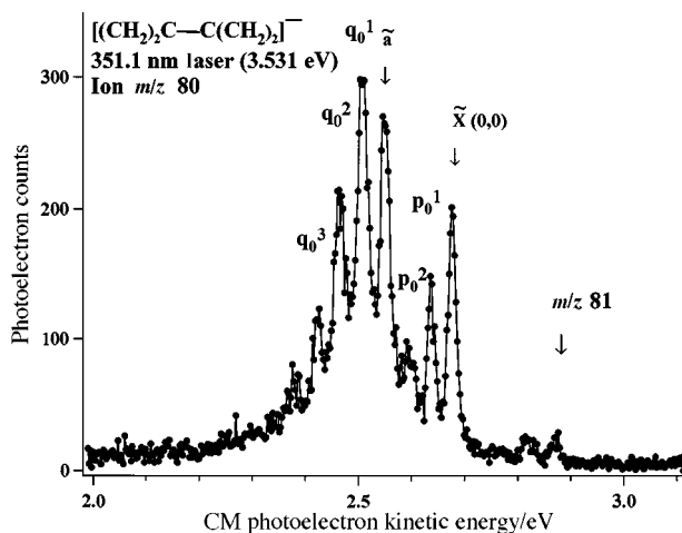
Fig. 2 A plot of the negative ion spectrum of the [(\text{CH}_2)_2\text{C}-\text{C}(\text{CH}_2)_2]^- ion, m/z 80; detachment laser \lambda_0 = 351.1 nm (3.531 eV). Because of imperfect mass-resolution this spectrum is slightly contaminated with peaks due to the [\text{CH}_2=\text{C}(\text{CH}_3)-\text{C}(\text{CH}_2)_2]^- ion at m/z 81.
