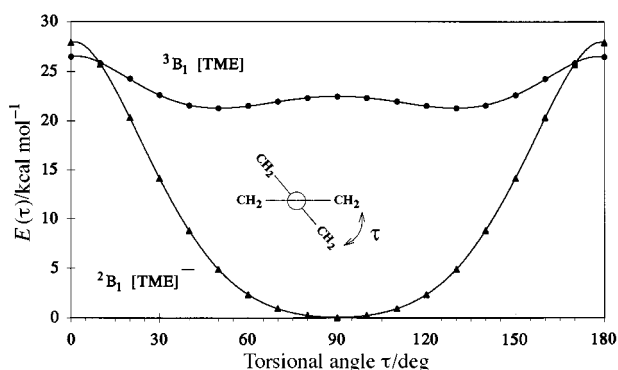
Fig. 7 Twisting potential energy curves [B3LYP/6-31+G(d)] of TME ^3B_1 and TME ^2B_1 with all geometrical parameters (except the dihedral angle, \tau ) held fixed at the equilibrium structure
