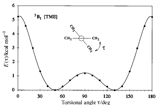
Fig. 6 Twisting potential energy curve [B3LYP/6-31+G(d)] of TME ^3B_1 with all geometrical parameters (except the dihedral angle, \tau ) held fixed at the equilibrium structure
