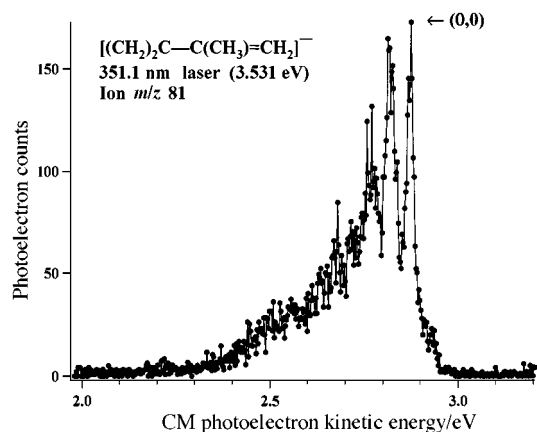
Fig. 1 A plot of the negative ion spectrum of the [\text{CH}_2=\text{C}(\text{CH}_3)-\text{C}(\text{CH}_2)_2]^- ion, m/z 81; detachment laser \lambda_0 = 351.1 nm (3.531 eV)
