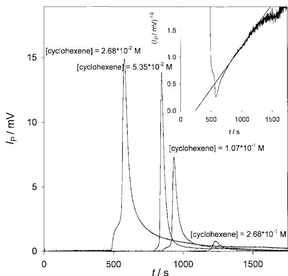
Fig. 6 I_p(t) as a function of time of the system TCNP–cyclohexene– H_2O_2 in THF at different cyclohexene concentrations. The inset presents the plot of 1/\sqrt{I_p(t)} versus time {see text} for [cyclohexene] = 2.68 \times 10^{-2} \text{ mol dm}^{-3} . Conditions: [TCNP] = 5.35 \times 10^{-2} \text{ mol dm}^{-3} ; [H_2O_2] = 5.35 \times 10^{-1} \text{ mol dm}^{-3} ; T = 20^\circ\text{C} . M denotes the concentration in \text{mol dm}^{-3} .
