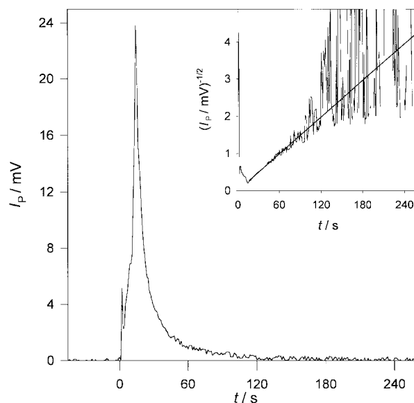
Fig. 9 I_p(t) as a function of time of the system CDT–1,2-epoxycyclohexane–H 2 O 2 in THF. The inset shows the corresponding plot of 1/\sqrt{I_p(t)} versus time. Conditions: [CDT] = 2.5 \times 10^{-2} mol dm -3 ; [1,2-epoxycyclohexane] = 2.5 \times 10^{-1} mol dm -3 ; [H 2 O 2 ] = 2.5 \times 10^{-1} mol dm -3 ; T = 20 °C.
