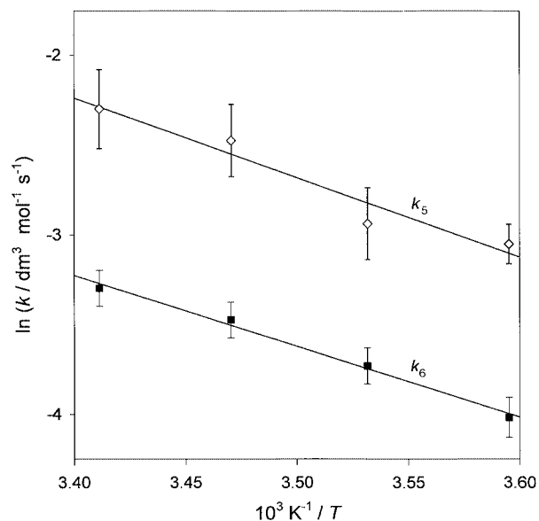
Fig. 3 Plots of \ln k_5 and \ln k_6 versus 1/T of the system CDT–H 2 O 2 in THF; with k_5 = k_f'(\text{CDT}) and k_6 = k_s'(\text{CDT}) {see text}. Conditions: [CDT] = 1.25 \times 10^{-2} mol dm -3 ; [H 2 O 2 ] = 1.25 \times 10^{-1} mol dm -3 .
