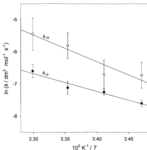
Fig. 5 Plots of \ln k_{18} and \ln k_{19} versus 1/T of the system TCNP–H 2 O 2 in THF; with k_{18} = k_f(\text{TCNP}) and k_{19} = k_s(\text{TCNP}) {see text}. Conditions: [TCNP] = 5.2 \times 10^{-2} mol dm -3 ; [H 2 O 2 ] = 5.2 \times 10^{-1} mol dm -3 .
