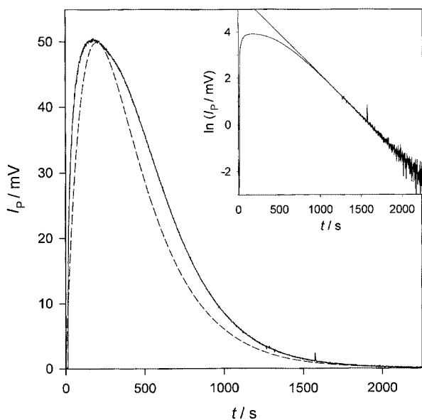
Fig. 1 I_p(t) as a function of time of the system CDT–H 2 O 2 in THF. The inset shows the corresponding plot of \ln I_p(t) versus time. Conditions: [CDT] = 1.25 \times 10^{-2} mol dm -3 ; [H 2 O 2 ] = 1.25 \times 10^{-1} mol dm -3 ; T = 10^\circ\text{C} . — = experimental curve; ---- = theoretically calculated curve according to eqn. (8) using c_1 = (3.0 \pm 0.2) \times 10^{11} mV dm 3 s mol -1 ; k_p = (0.45 \pm 0.10) s -1 and \tau_A = (18 \pm 1) \mu\text{s} ; k_f'(\text{CDT}) = 7.2 \times 10^{-3} s -1 ; k_s'(\text{CDT}) = 3.4 \times 10^{-3} s -1 .
