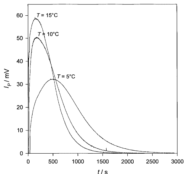
Fig. 2 Plots of I_p(t) versus t of the system CDT–H 2 O 2 in THF determined at three different temperatures. Conditions: [CDT] = 1.25 \times 10^{-2} mol dm -3 ; [H 2 O 2 ] = 1.25 \times 10^{-1} mol dm -3 .
