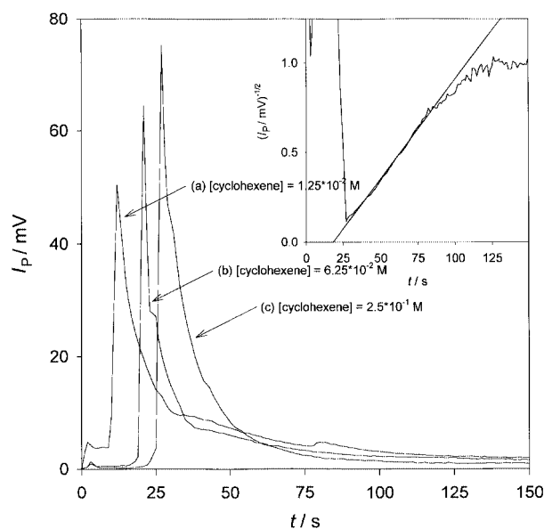
Fig. 7 I_p(t) as a function of time of the system CDT–cyclohexene– H_2O_2 in THF at different cyclohexene concentrations. The inset shows the plot of 1/\sqrt{I_p(t)} versus time for the system (c). Conditions: [CDT] = 2.5 \times 10^{-2} \text{ mol dm}^{-3} ; [H_2O_2] = 2.5 \times 10^{-1} \text{ mol dm}^{-3} ; T = 10^\circ\text{C} . M denotes the concentration in \text{mol dm}^{-3} .
