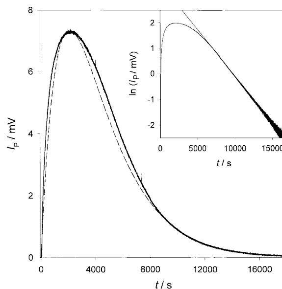
Fig. 4 I_p(t) as a function of time of the system TCNP-H 2 O 2 in THF. The inset shows the corresponding plot of \ln I_p(t) versus time. Conditions: [TCNP] = 5.2 \times 10^{-2} \text{ mol dm}^{-3} ; [H 2 O 2 ] = 5.2 \times 10^{-1} \text{ mol dm}^{-3} ; T = 20^\circ\text{C} . — = experimental curve; ---- = theoretically calculated curve according to eqn. (8) using c_2 = (1.4 \pm 0.1) \times 10^{11} \text{ mV dm}^3 \text{ s mol}^{-1} ; k_p = (0.45 \pm 0.10) \text{ s}^{-1} and \tau_A = (15 \pm 1) \mu\text{s} ; k_f'(\text{TCNP}) = 5.9 \times 10^{-4} \text{ s}^{-1} ; k_s'(\text{TCNP}) = 3.7 \times 10^{-4} \text{ s}^{-1} .
