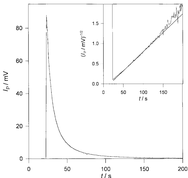
Fig. 8 I_p(t) as a function of time of the system CDI–H 2 O 2 in THF. The inset shows the corresponding plot of 1/\sqrt{I_p(t)} versus time. Conditions: [CDI] = 2.5 \times 10^{-2} mol dm -3 ; [H 2 O 2 ] = 2.5 \times 10^{-1} mol dm -3 ; T = 10 °C.
