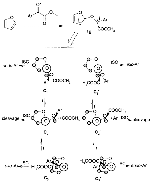
Scheme 4
