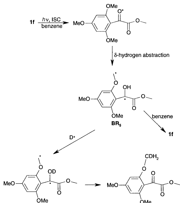
Scheme 9
