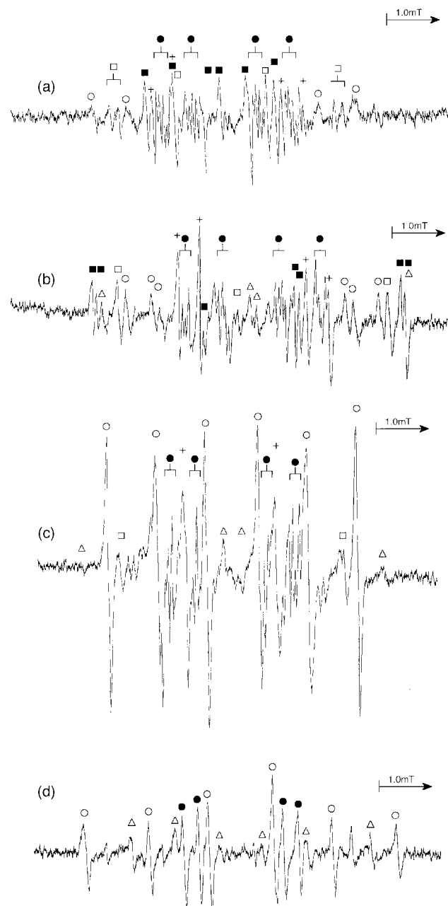
Fig. 2 EPR spectra observed for the reaction between SO _4^{\cdot-} and the following compounds at pH ca. 2.5: (a) \alpha -D-glucose (0.017 mol dm ^{-3} ), + ( 6 ), \square ( 7 ), \circ ( 8 ), \bullet ( 9 ), \blacksquare ( 10 ); (b) \beta -D-glucose (0.017 mol dm ^{-3} ), + ( 6 ), \square ( 13 ), \triangle ( 14 ), \circ ( 15 ), \bullet ( 16 ), \blacksquare ( 17 ); (c) sucrose (0.017 mol dm ^{-3} ), \square ( 18 ), \triangle ( 19 ), \bullet ( 20 ), + ( 21 ), \circ ( 22 ); (d) D-fructose (0.033 mol dm ^{-3} ), \triangle ( 1 ), \circ ( 23 ), \bullet ( 24 ).
