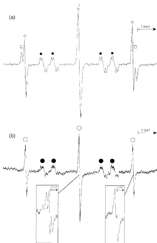
Fig. 4 EPR spectrum observed for the reaction of myo -inositol (0.033 mol dm ^{-3} ) at pH ca. 2.5 with: (a) HO \cdot , \circ ( 26 ) and ( 31 ), \bullet ( 27 ) and ( 28 ), \square ( 29 ) and ( 30 ); (b) SO _4^{\cdot-} , \circ ( 26 ), \bullet ( 27 ) and ( 28 ), with inset, signals obtained under photolytic conditions (see text).
