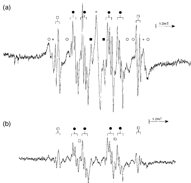
Fig. 3 EPR spectra observed for the reaction of starch (water soluble, 1%) at pH ca. 2.5 with: (a) HO \cdot , \square C ^2 , \triangle C ^3 , + C ^4 , \circ C ^5 , \bullet C ^6 ; (b) SO _4^{\cdot-} , \square C ^2 , \bullet C ^6 .
