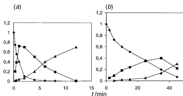
Fig. 1 (a) Decomposition of lomefloxacin ( 3 ) (◆) and formation of products 11 (■) and 10 (●) by irradiation of an aqueous solution 0.2 M in NaCl at pH 7.2. (b) The same in 0.1 M HCl.
