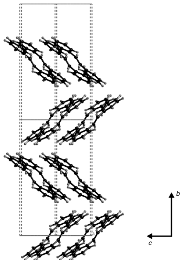
Fig. 2 Model structure used to simulate electron diffraction patterns.
