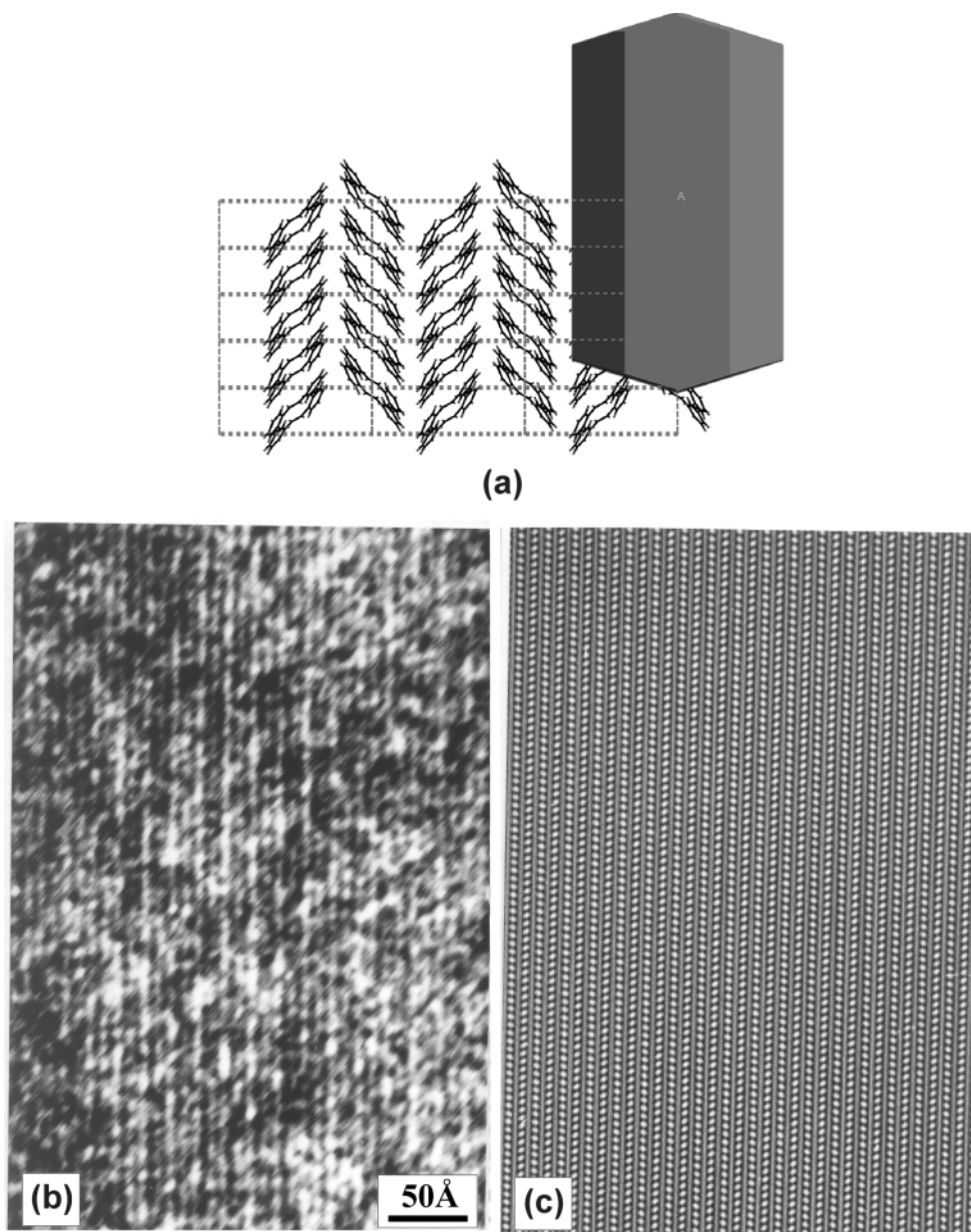
Fig. 5 Model structure (a) with high resolution image (b) and simulated image (c).
