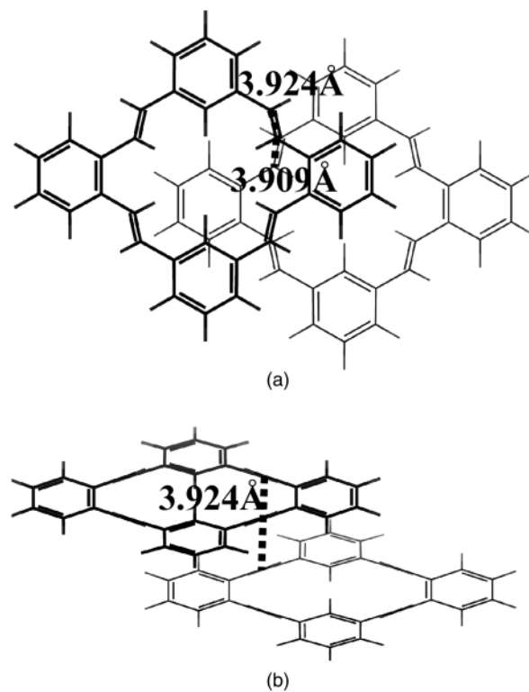
Fig. 13 Intrastack dimer in C_1 symmetry ( ab initio calculations), (a) top view; (b) side view.
