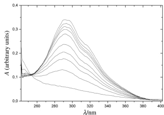
Fig. 16 Reaction spectra of the monochromatic irradiation ( \lambda = 366 \text{ nm} ) of 8 in \text{CHCl}_3 : the maximum of the absorbance A at 292 \text{ nm} decreases almost completely within 1 h.
