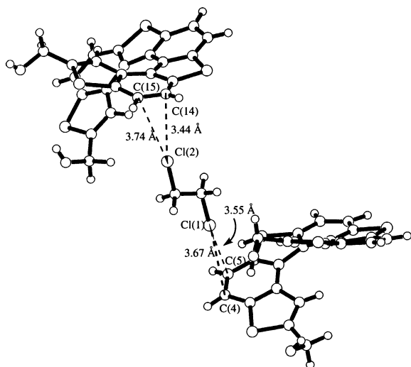
Fig. 6 Crystal structure of the clathrate (PM-1)_2 \cdot (1,2\text{-dichloroethane}) .
