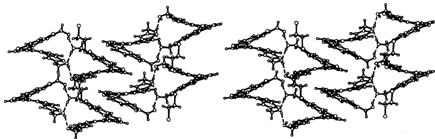
Fig. 5 Stereoview of the heterochiral dimer of P - and M -helicenediols in the clathrate (PM-1)_2 \cdot (1,2\text{-dichloroethane}) .
