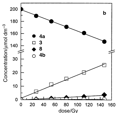
Fig. 5 Oxidation of 2a (insert a) and 4a (insert b) by reaction of radiolytically generated \text{Br}_2^{\bullet-} and formation of products at a dose rate of 2.5 \text{ Gy min}^{-1} at pH 7.4.
