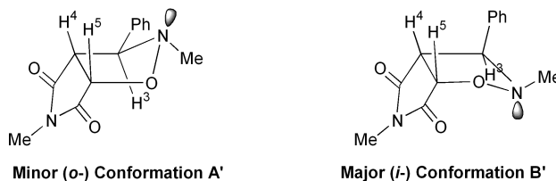
Fig. 2 Conformations of the adduct 5c .
