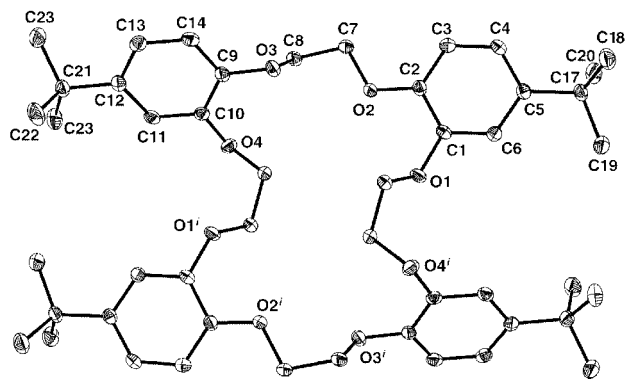
Fig. 2 ORTEP representation with 50% probability ellipsoids of 4,5',4'',5'''-tetra- tert -butyltetrabenzo-24-crown-8. Hydrogen atoms are omitted for clarity. Symmetry code i\ 2 - x, 2 - y, -z .
