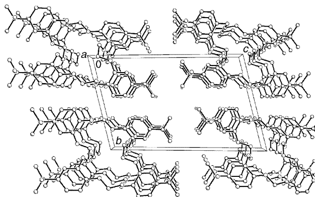
Fig. 3 Stacking diagram for 4,5',4'',5'''-tetra- tert -butyltetrabenzo-24-crown-8. Atoms are represented by circles and hydrogen atoms are omitted for clarity.
