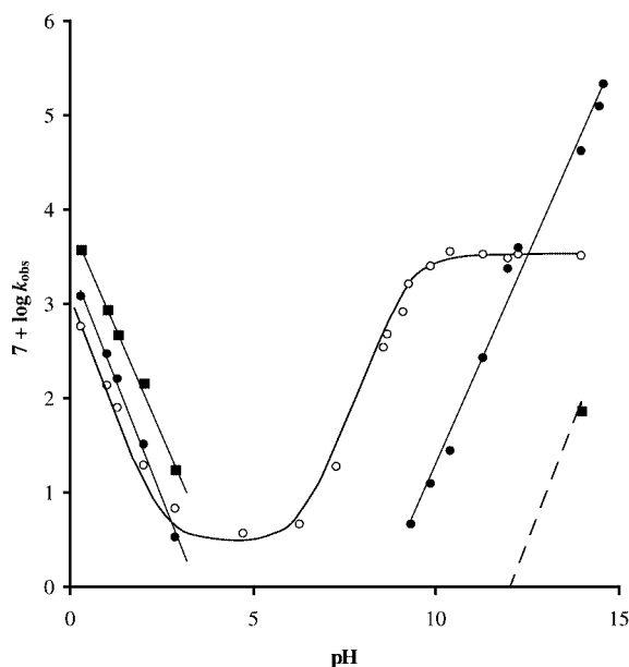
Fig. 1 pH-Rate profiles for the hydrolyses of: ●, 5a ; ○, 5b ; ■, 5c .
